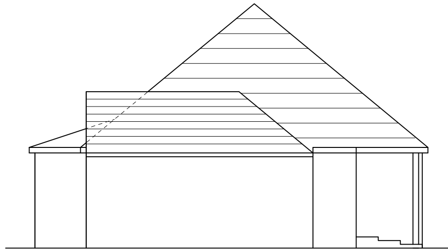
EXISTING SIDE ELEVATION 1
