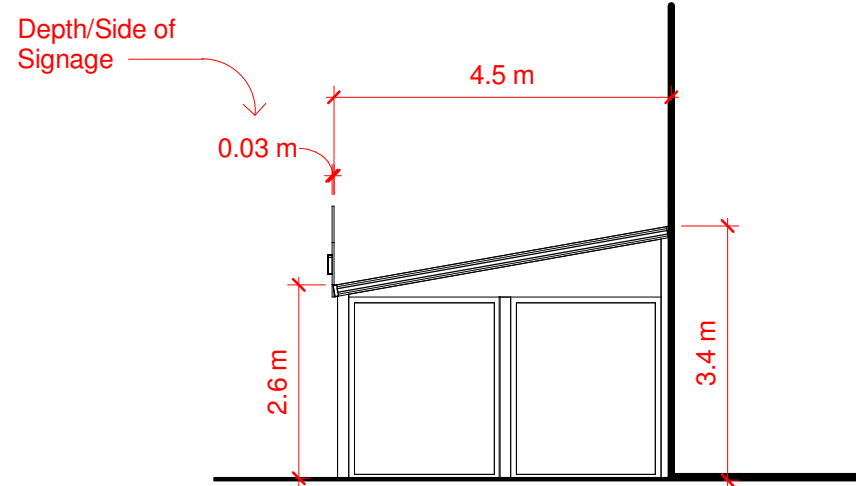
2 Elevation Side Elevation II 1 : 100
