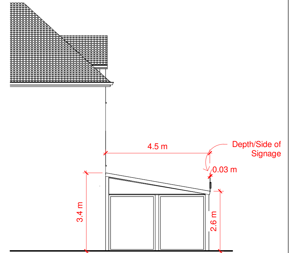
3 Elevation Side Elevation . 1 : 100
