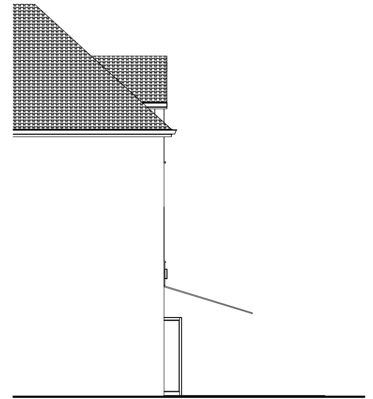
3 Pre-Elevation Side Elevation.. 1 : 100
