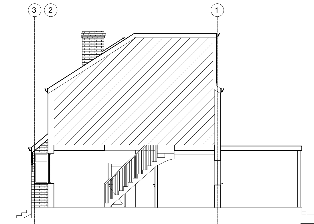
EXISTING SECTION
