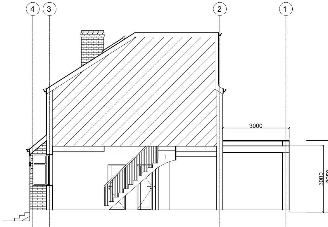
PROPOSED SECTION
