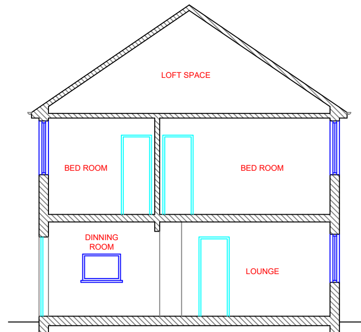
PRE-EXISTING SECTION A-A
