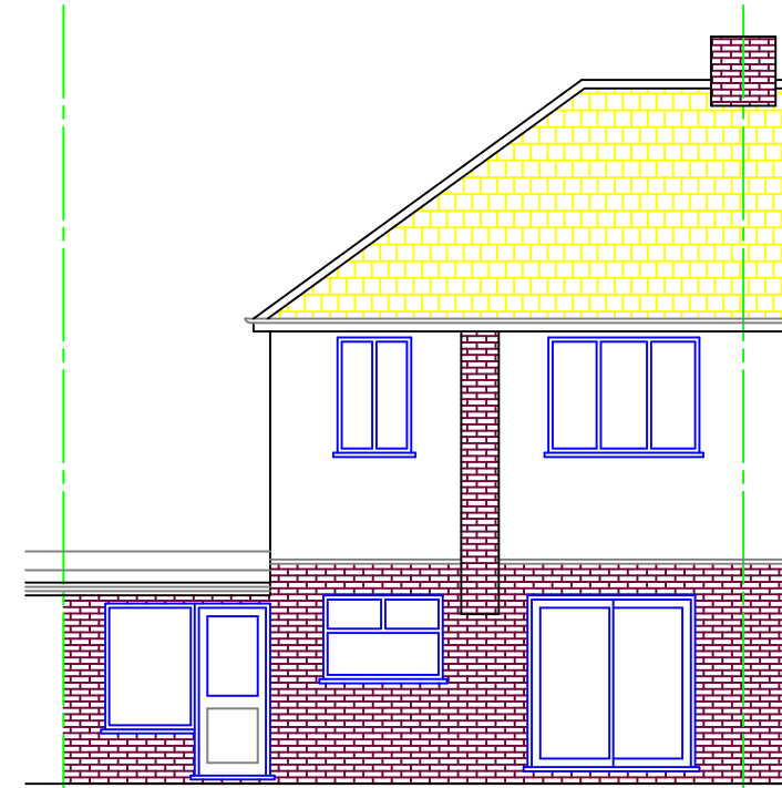
PRE-EXISTING REAR ELEVATION
