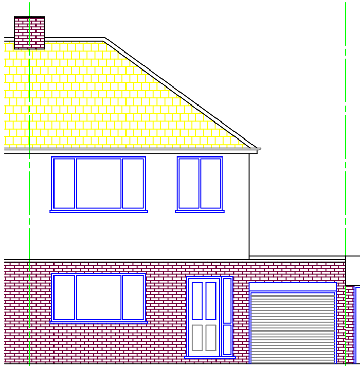
PRE-EXISTING FRONT ELEVATION
