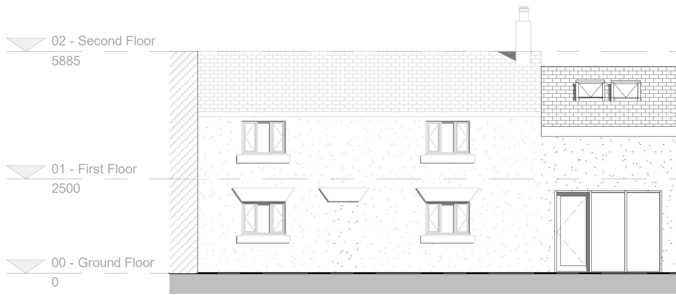
Front Elevation
