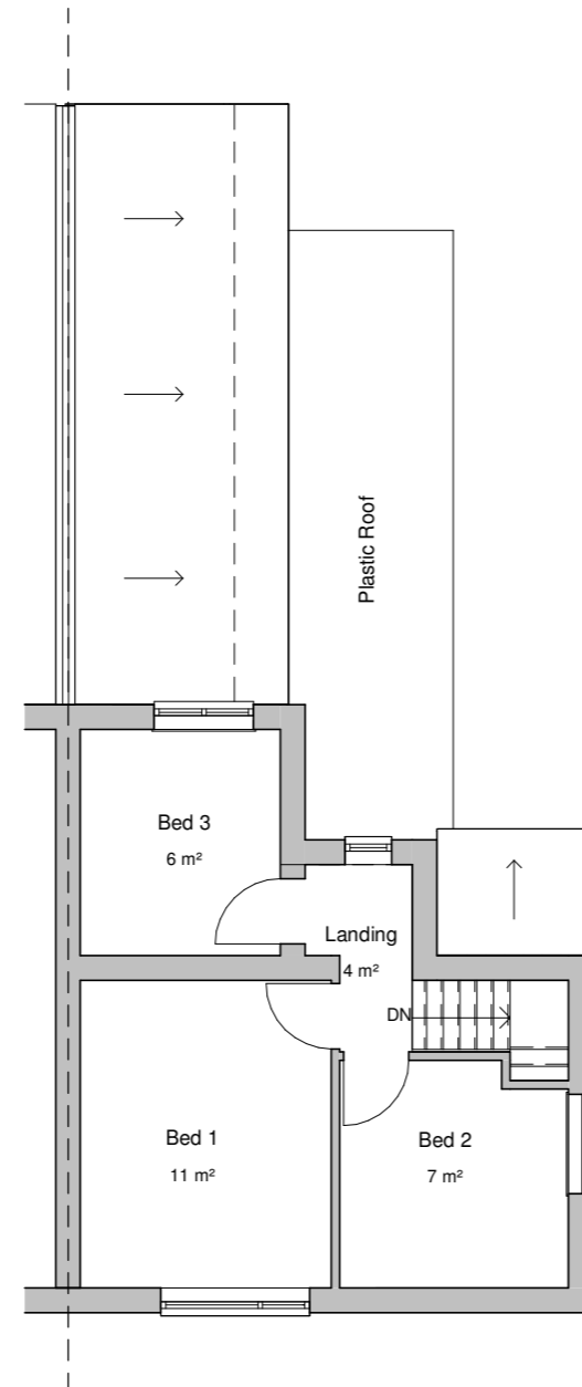
GA First Floor Plan As Existing 1 : 100
