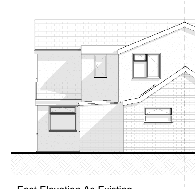
East Elevation As Existing 1 : 100
