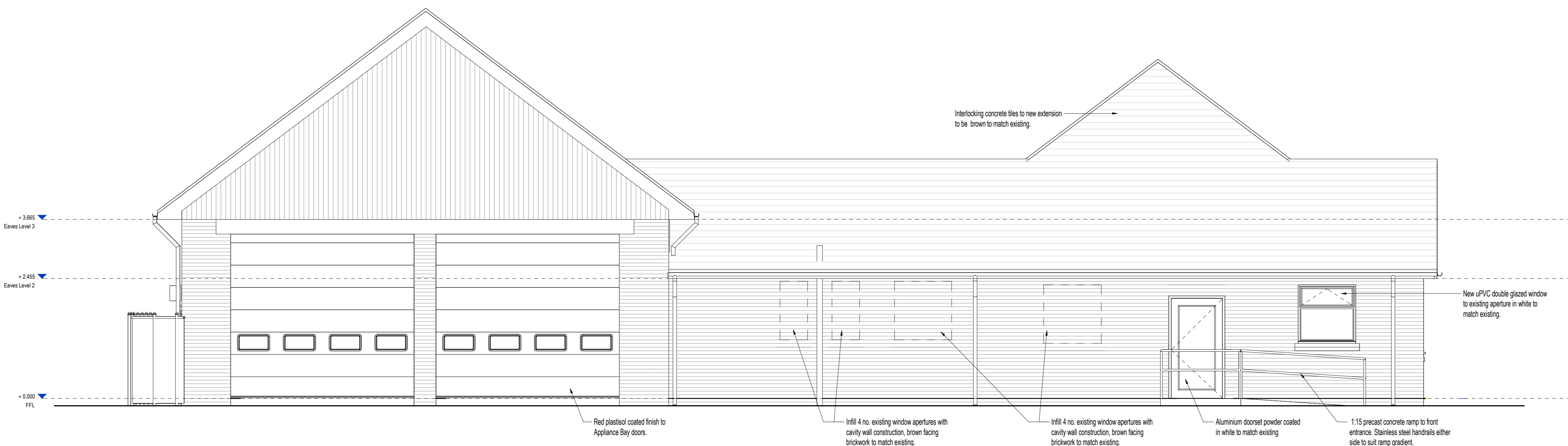
NW Elevation - Proposed 1:50
