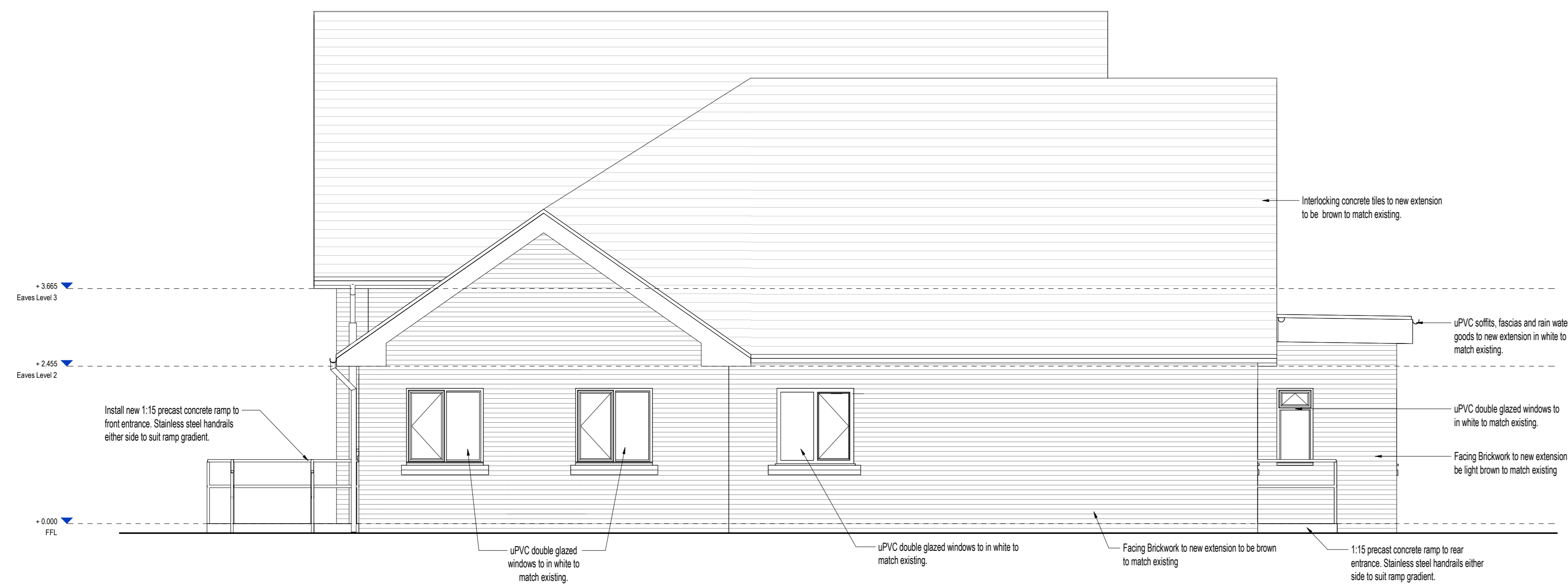
SW Elevation - Proposed 1:50
