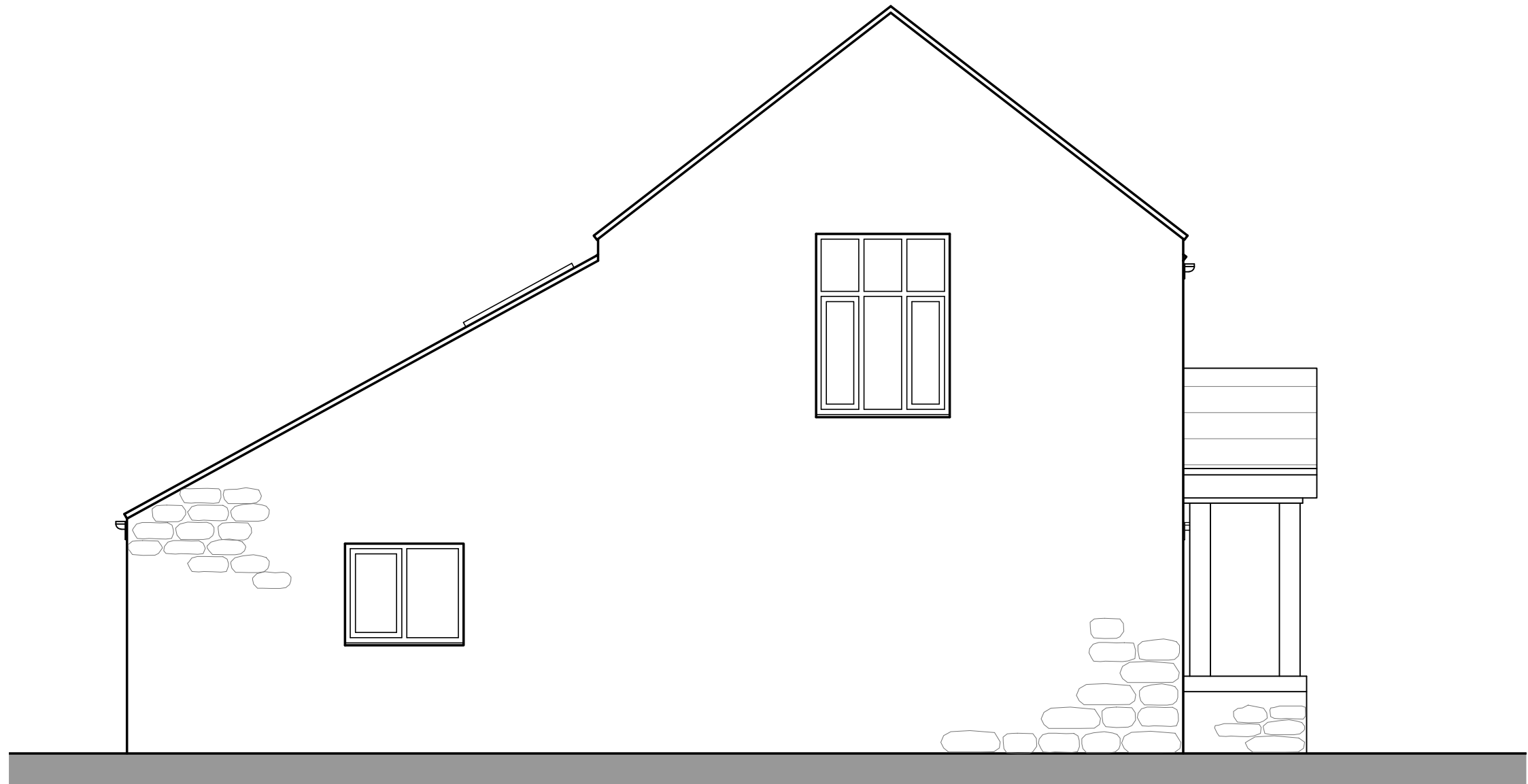
PROPOSED EAST (SIDE) ELEVATION
