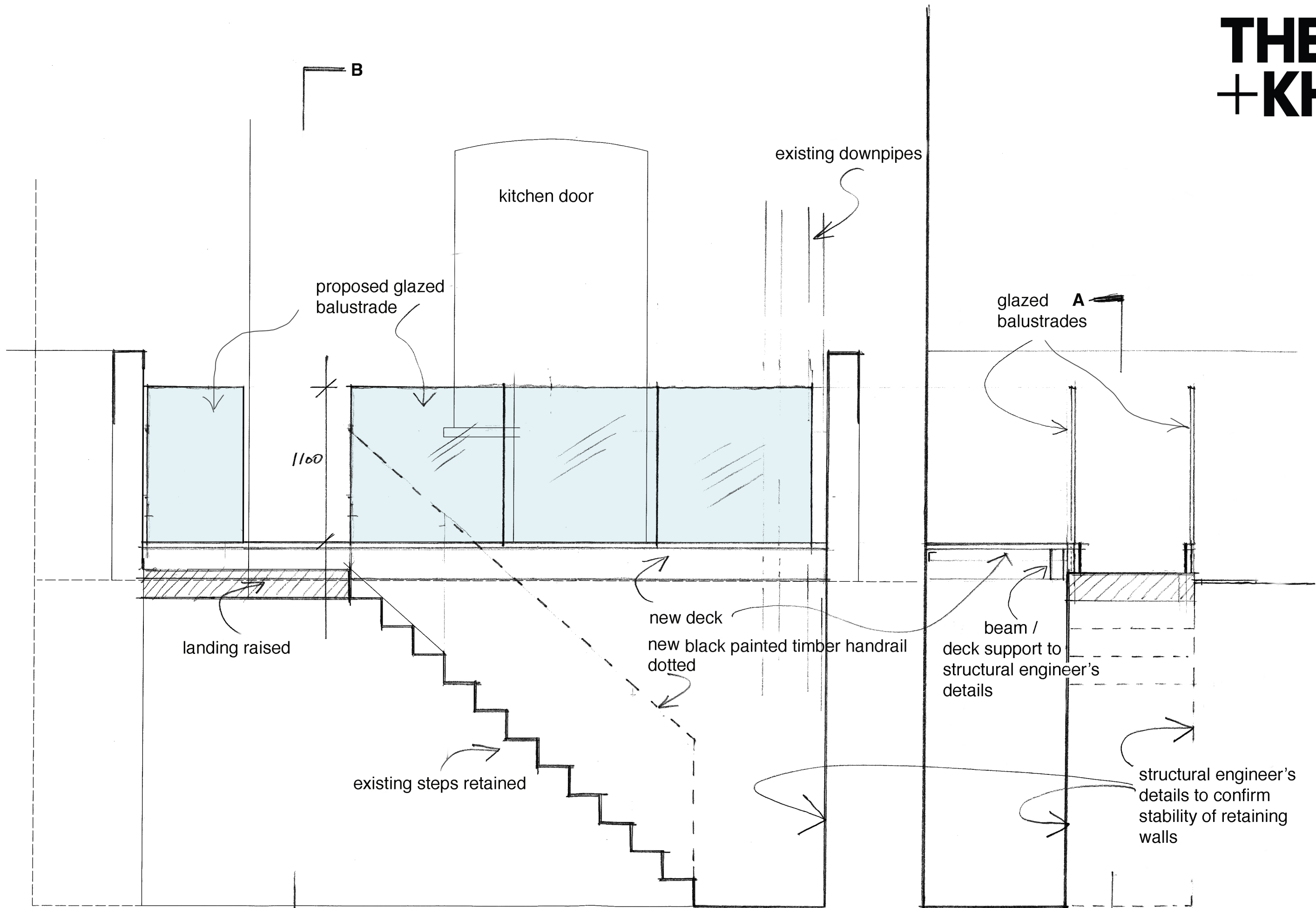
Section AA
