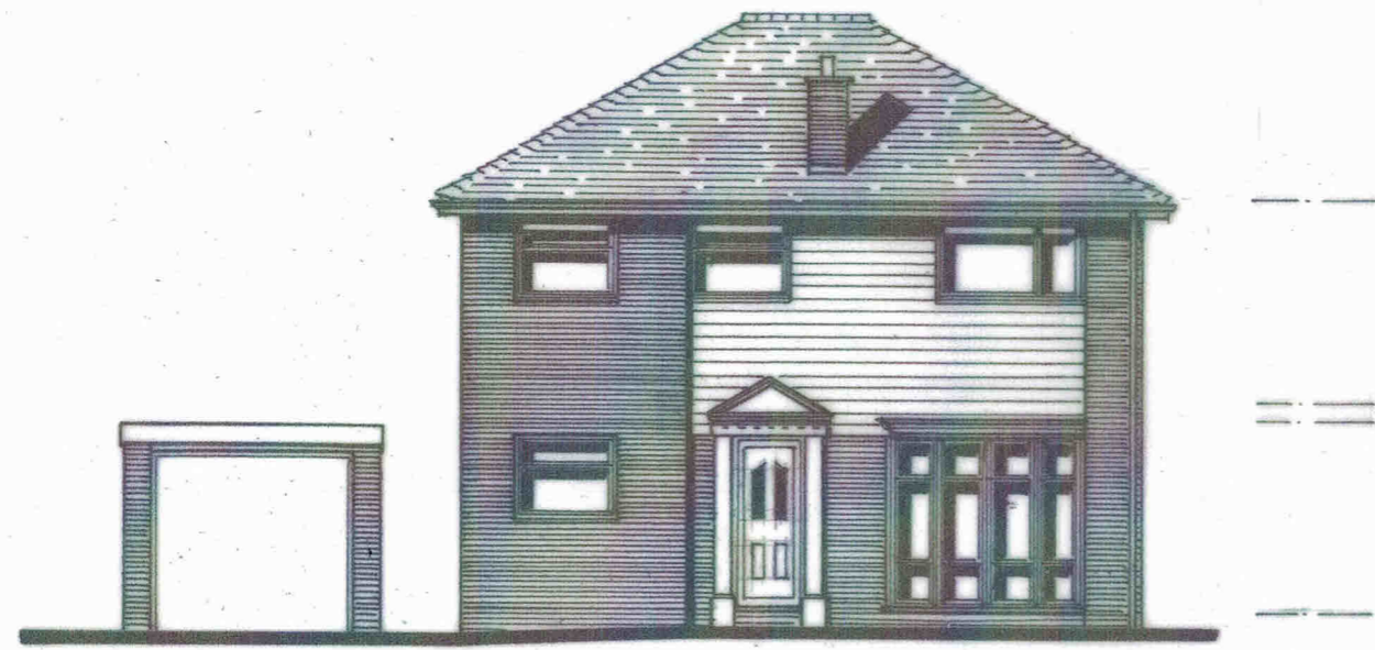
FRONT ELEVATION north 1:100
