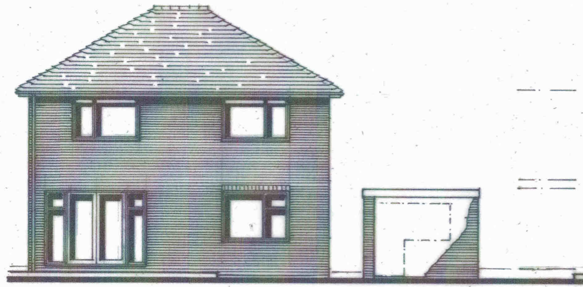
REAR ELEVATION south 1:100
