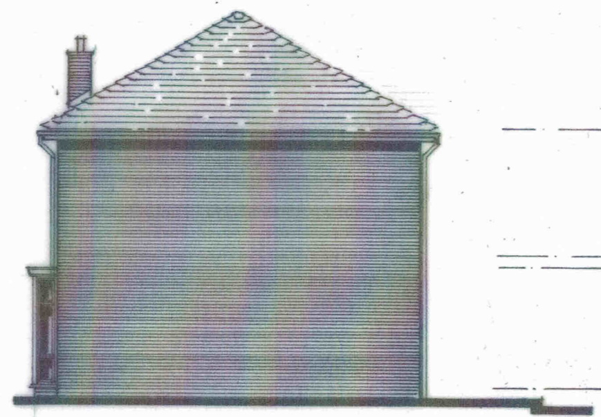
SIDE ELEVATION west 1:100
