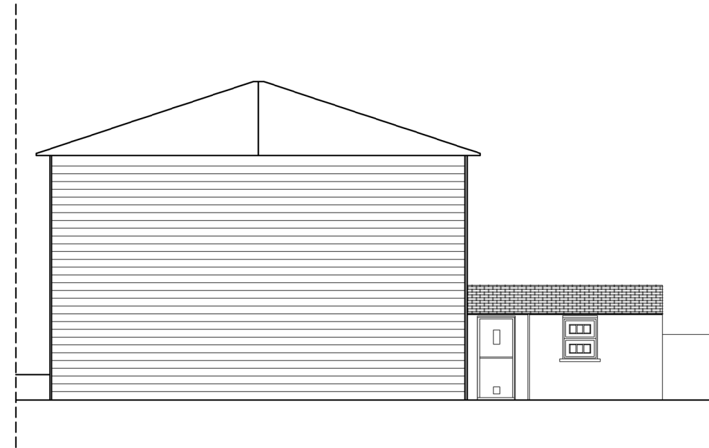
Proposed Right Hand Side Elevation 1:00 @ A3
