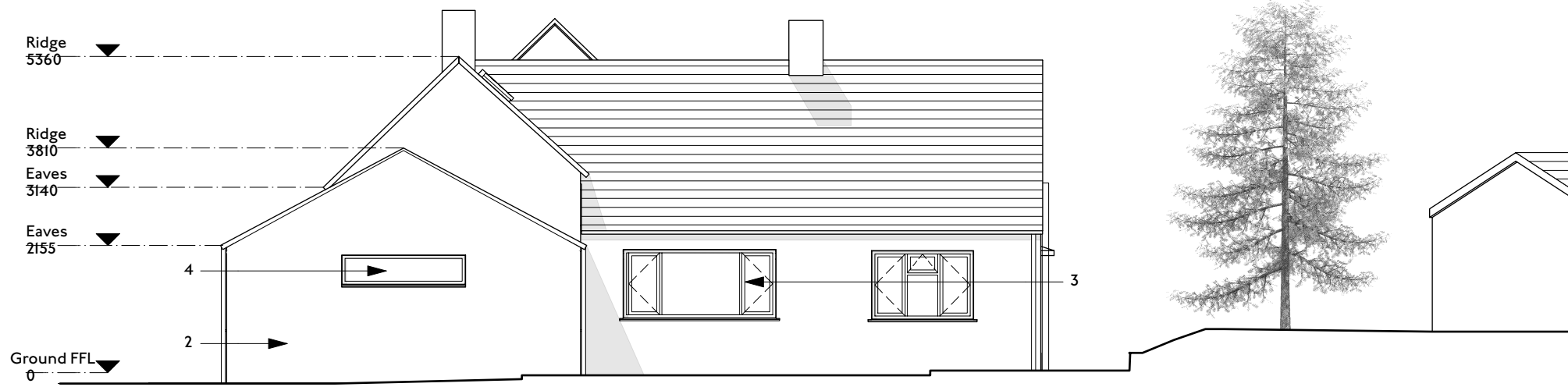
1 | 1:100 Proposed North-East Elevation
