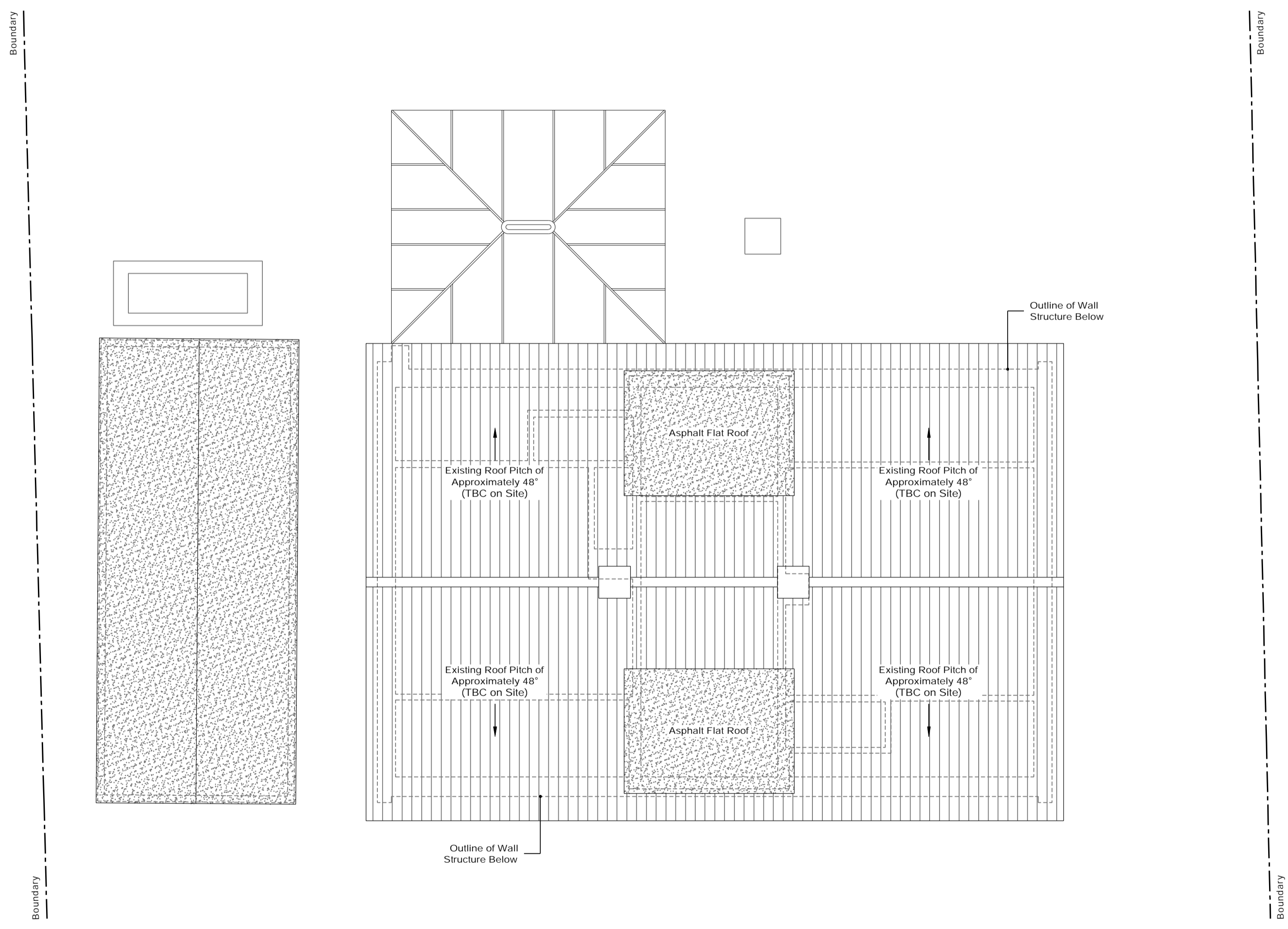
4.1 Existing Roof Covering Plan Scale 1:50
