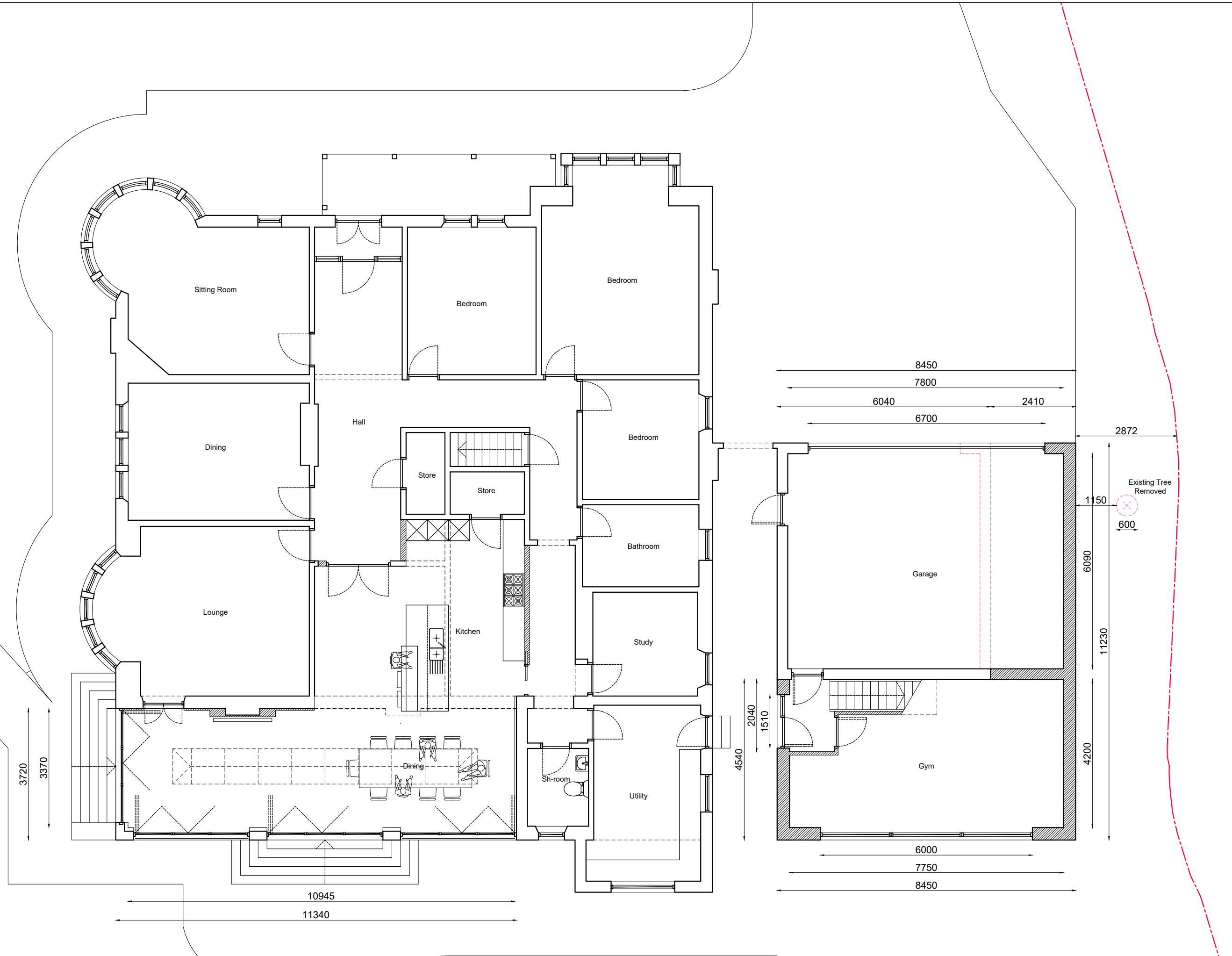
Ground Floor Plan as Proposed @ 1:100
