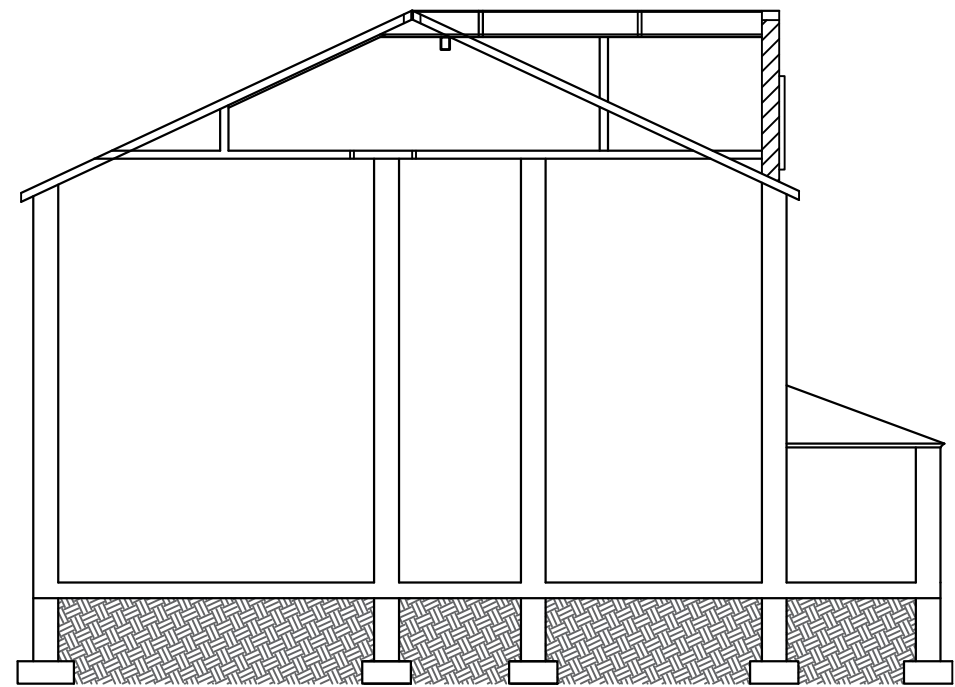
PROPOSED SECTION X -- X
