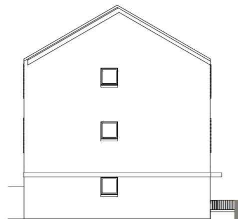
West Elevation
