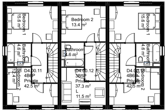
01_First Floor
