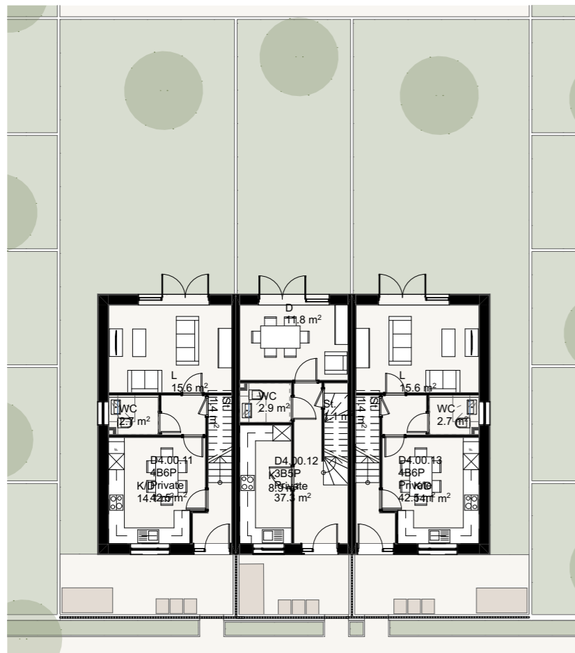
00_Ground Floor
