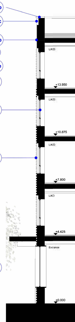
Block E Detail Section AA 1:50
