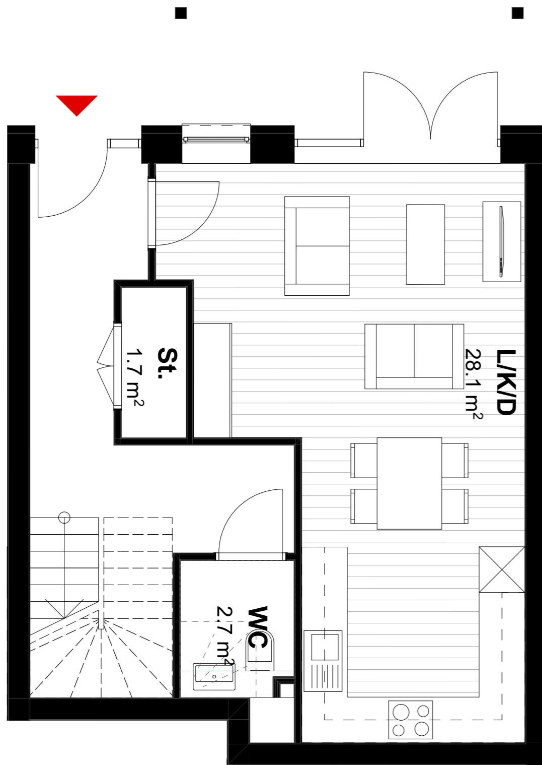
01_First Floor
