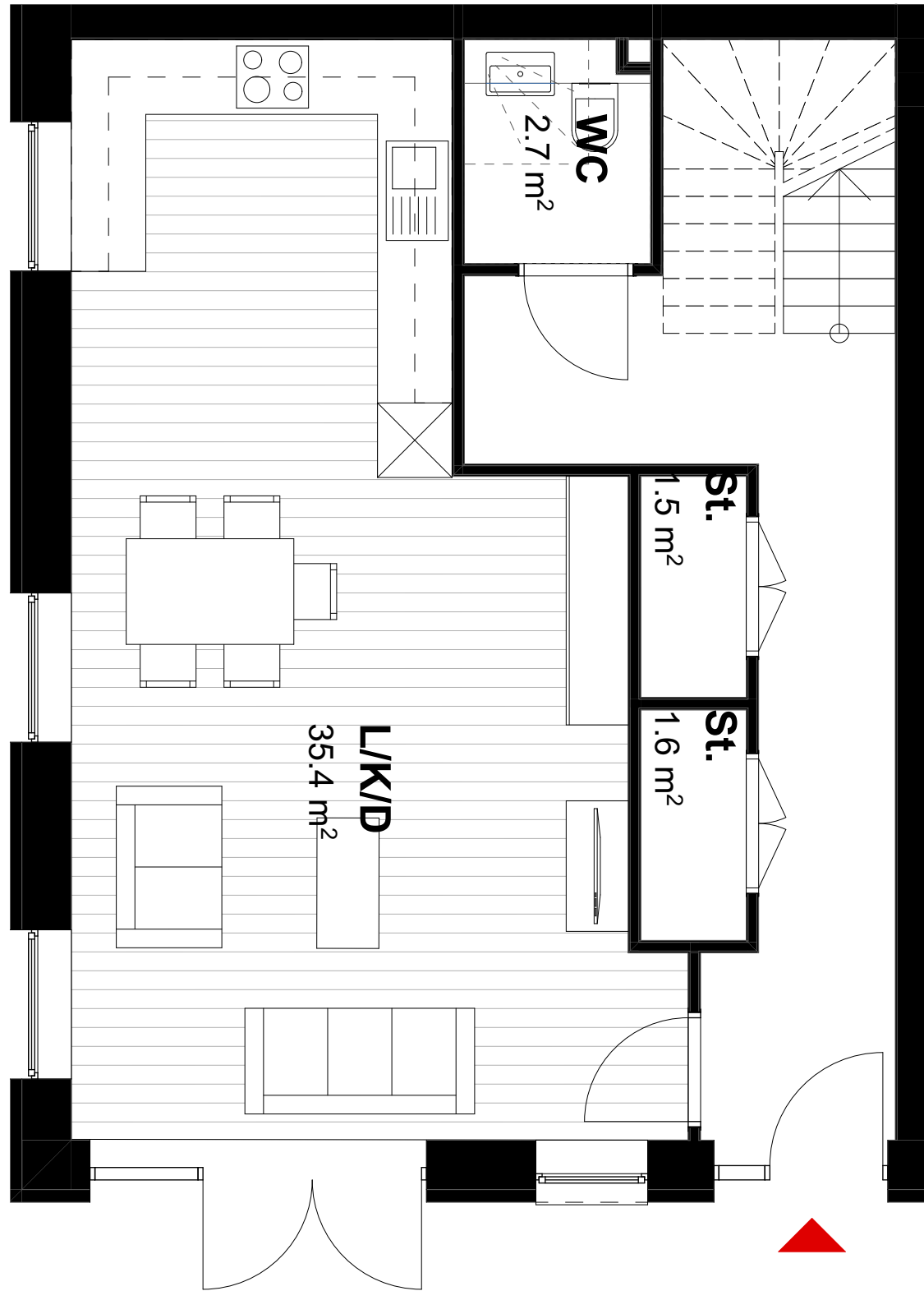
01_First Floor
