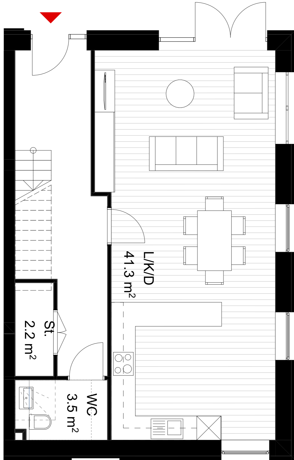
01_First Floor
