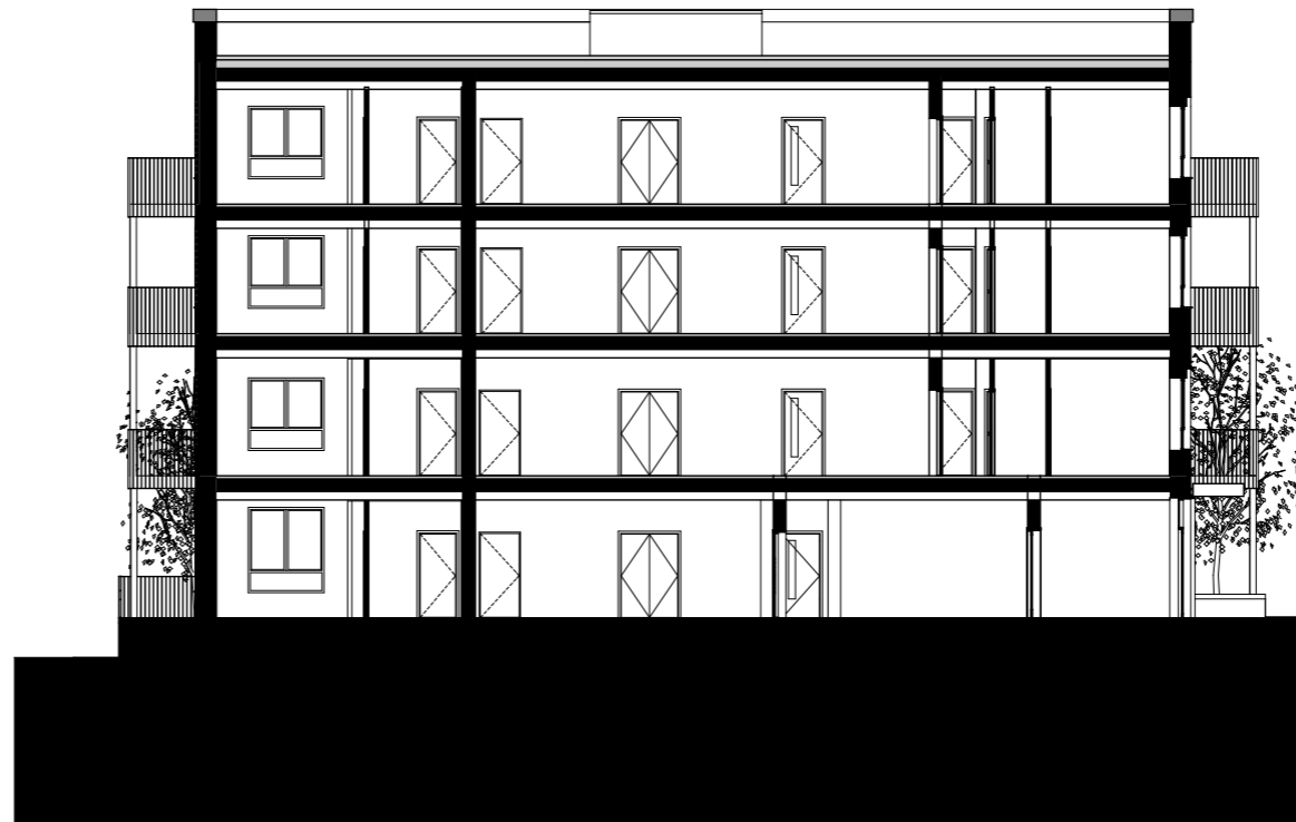
Block F Section bb 1:200
