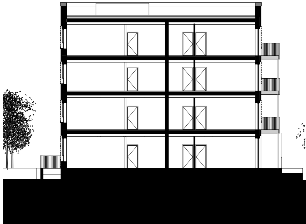
Block F Section aa 1:200
