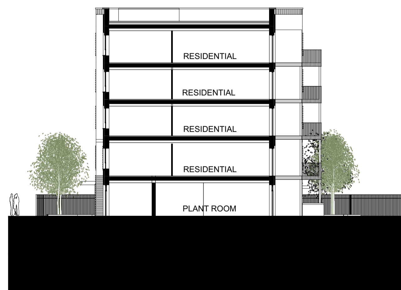
Block C Section bb 1:200
