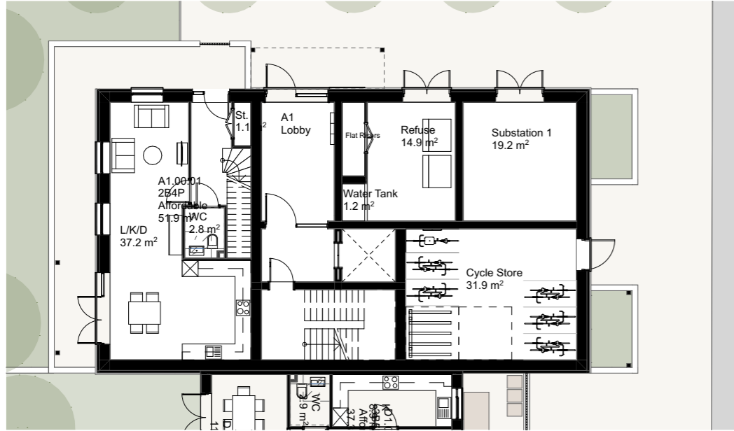
00_Ground Floor
