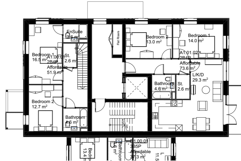
01_First Floor
