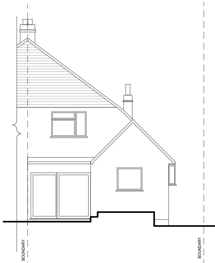
REAR ELEVATION
