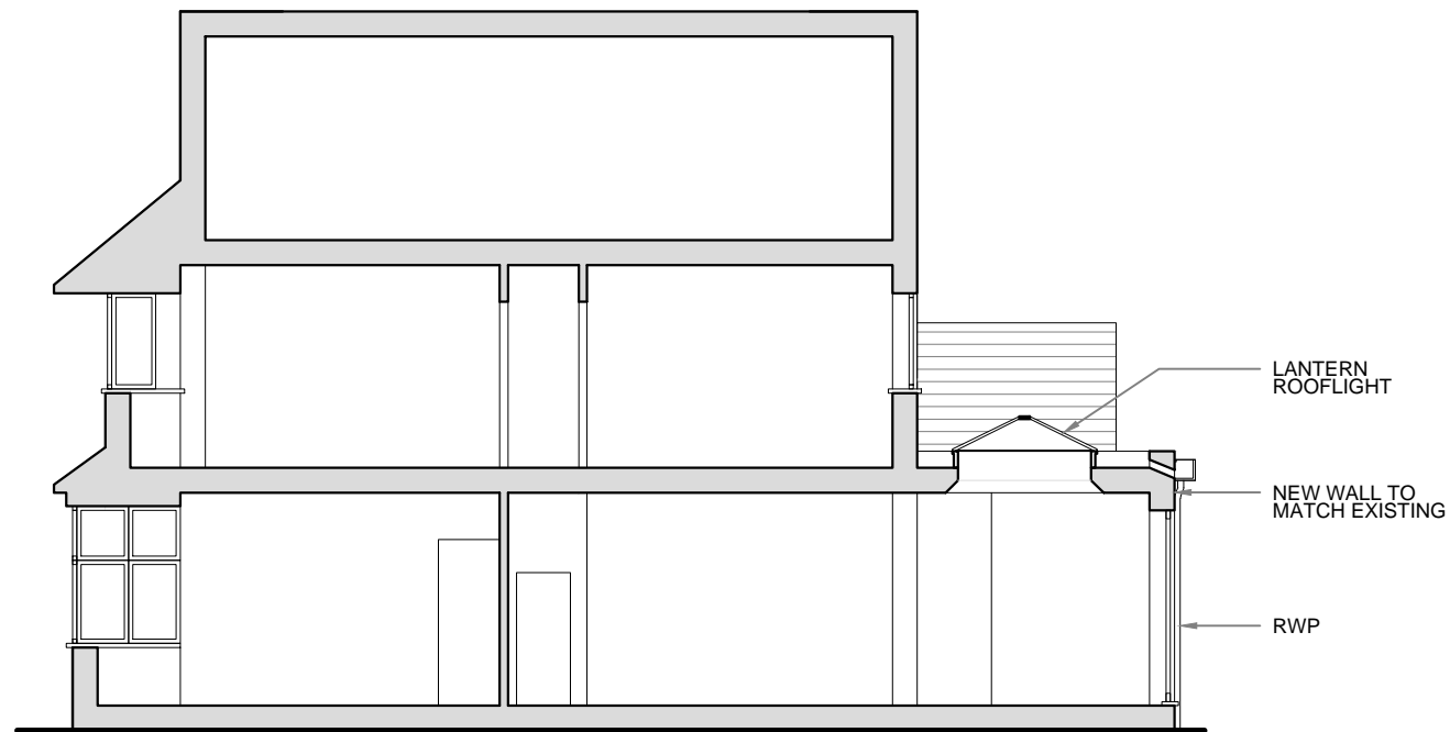
SECTION B-B
