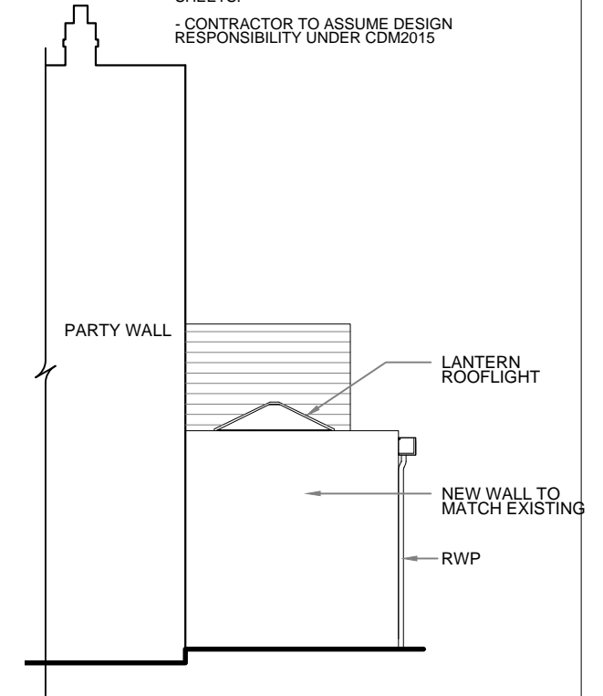
WEST ELEVATION
