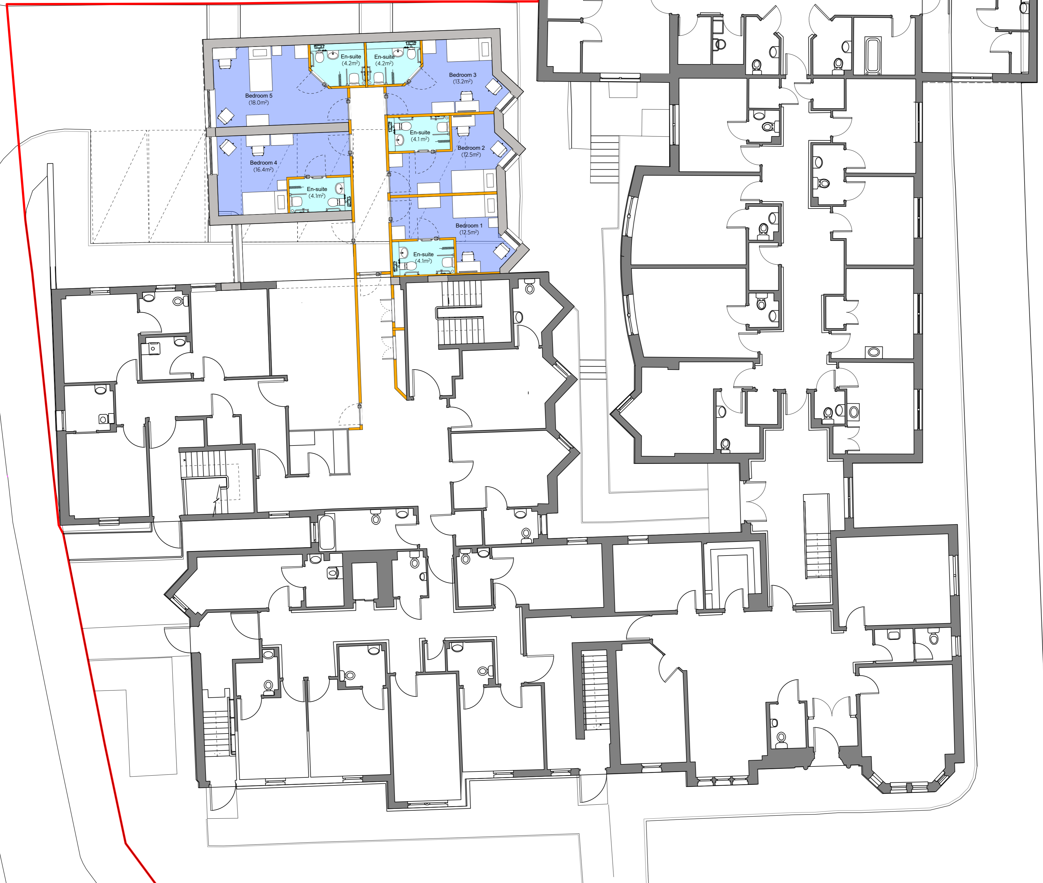
Proposed Ground Floor Layout SCALE 1:100
