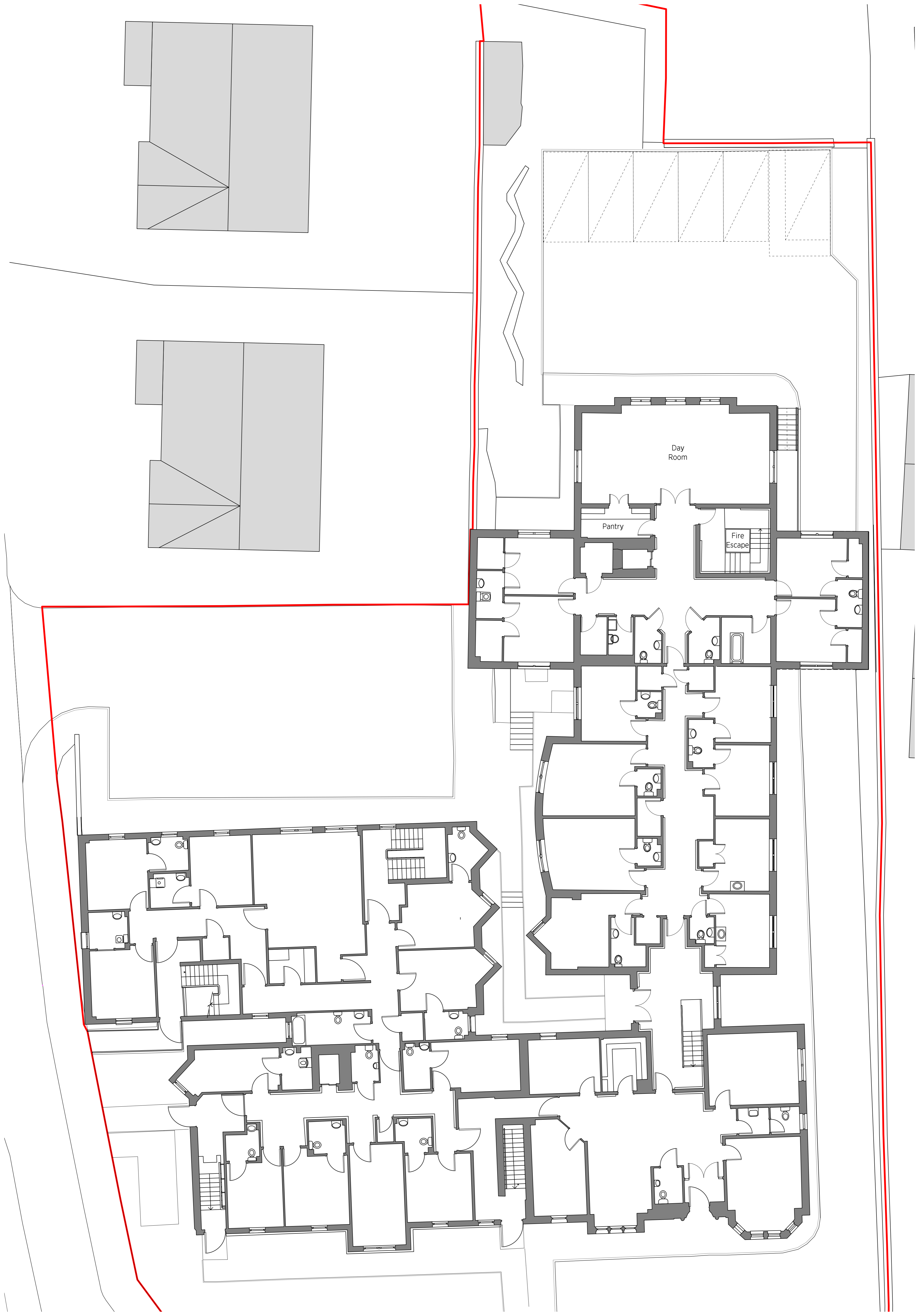
Existing Ground Floor Layout SCALE 1:100
