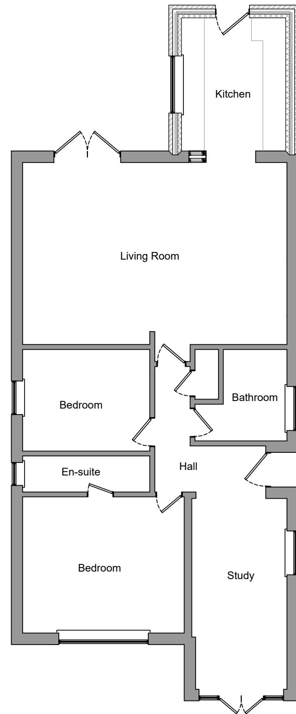
Ground Floor Layout 0 1m 2m Scale: 1:100
