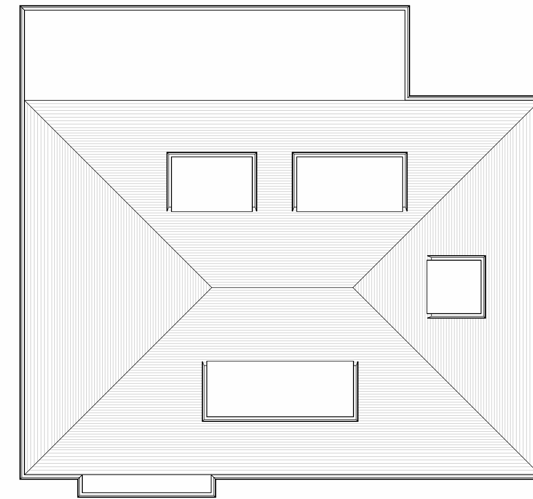
③ Existing Roof Plan 1:100
