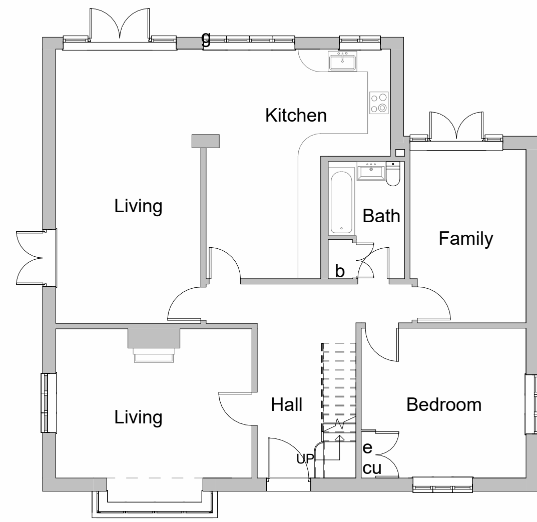
① Existing Ground Floor 1:100
