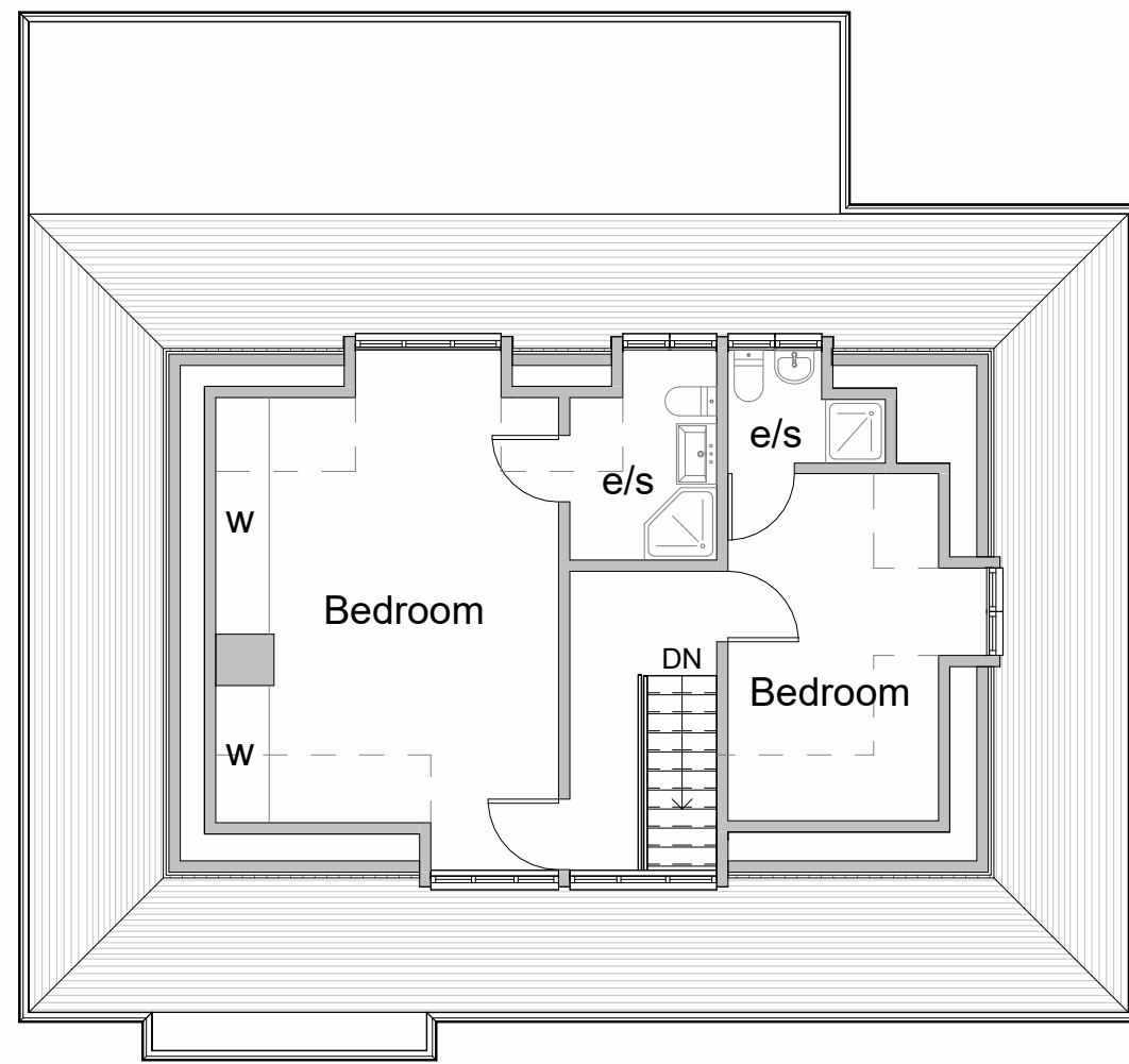
② Existing First Floor 1:100
