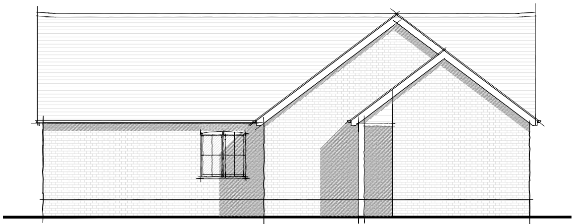
EAST ELEVATION 1:100
