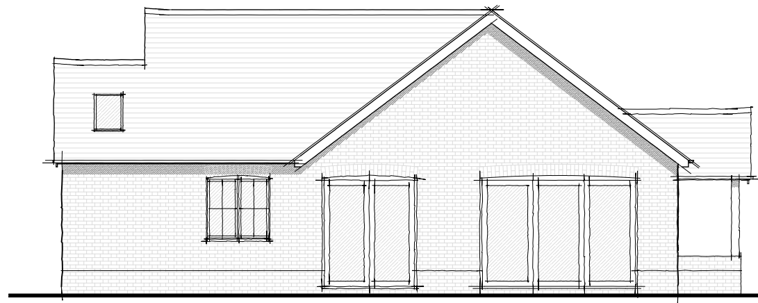
NORTH ELEVATION 1:100
