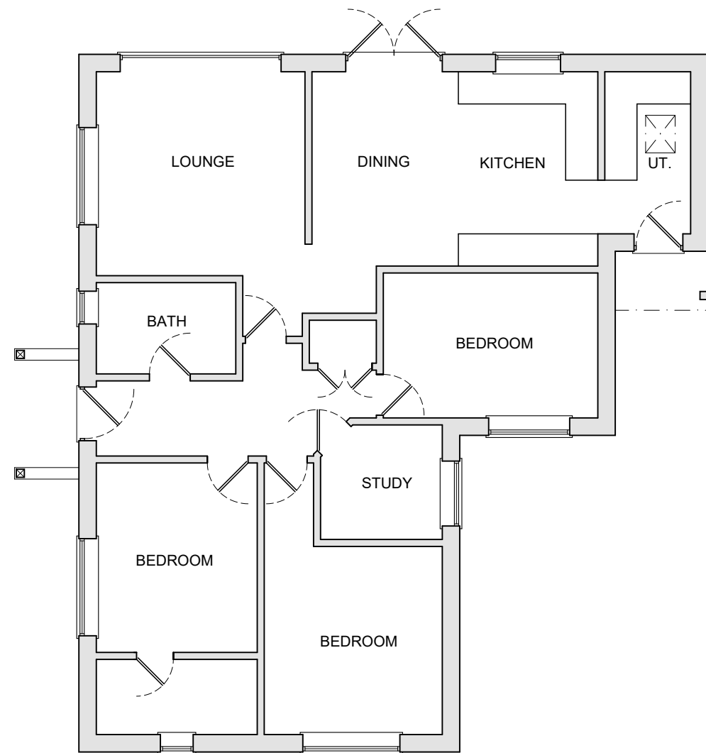
FLOOR PLAN 1:100
