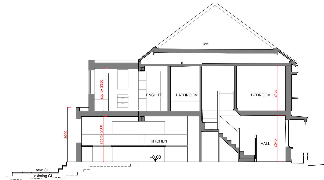
SECTION BB
