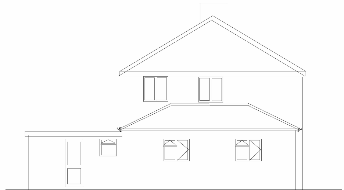
Proposed Side Elevation (Retrospective)
