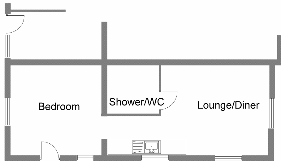
Proposed Ground Floor (Retrospective)
