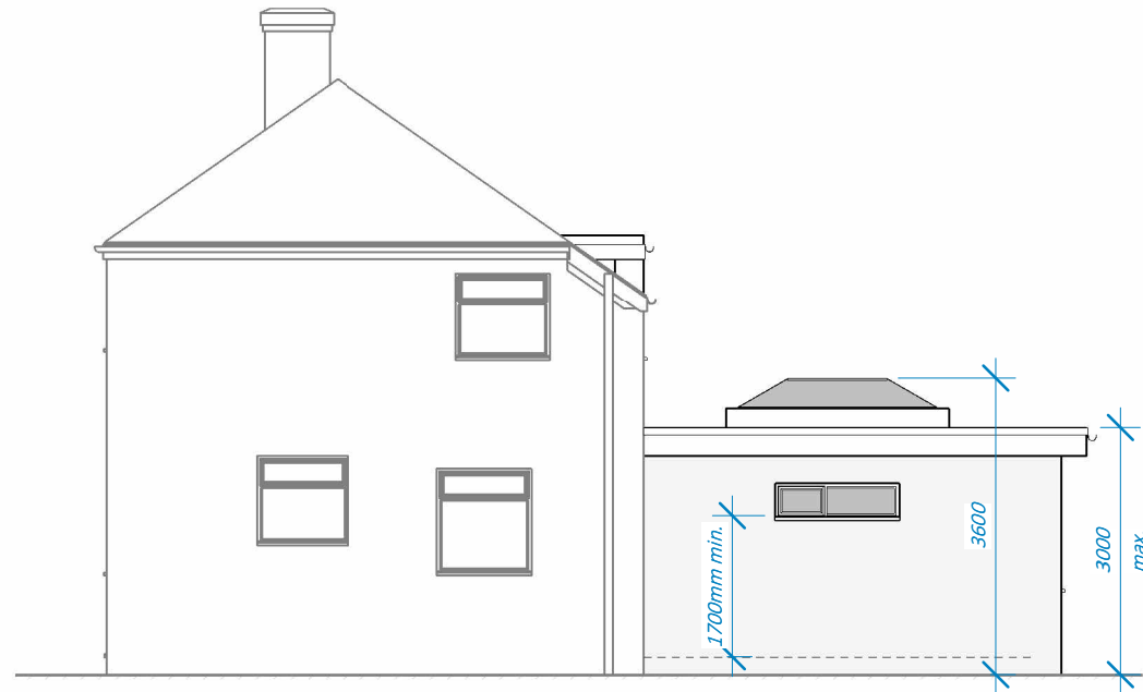
2 P05 north east elevation - proposed 1 : 100
