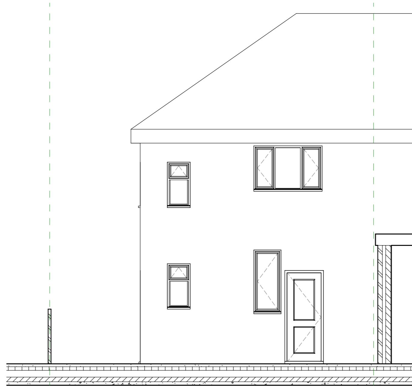
1 Existing Rear Elevation 1 : 50
