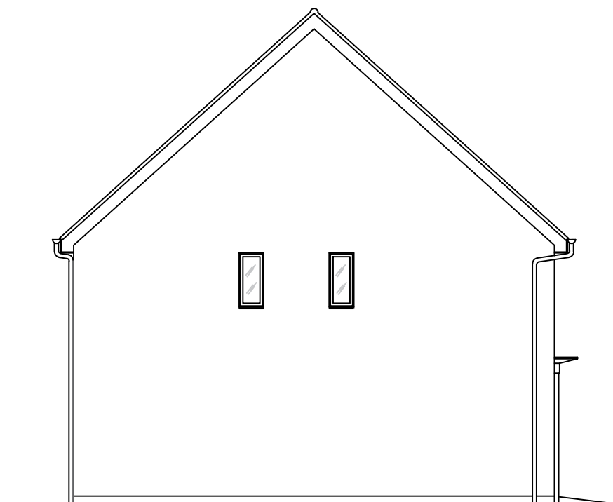
EXISTING SIDE (E) ELEVATION
