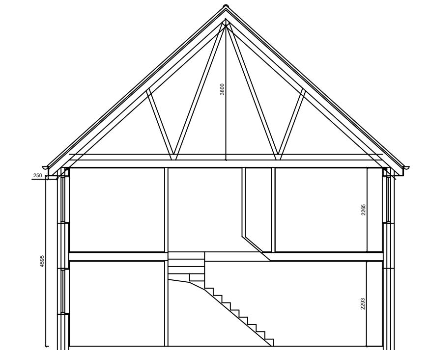
SECTION THROUGH
