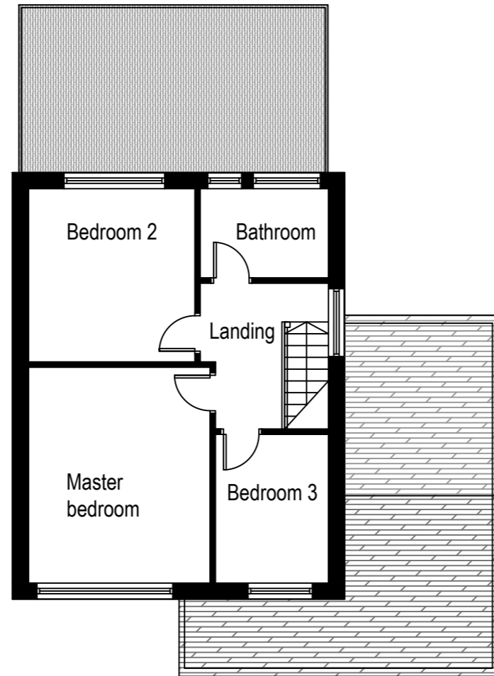
First floor plan @ 1:100 scale
