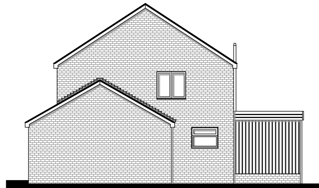
North Elevation @ 1:100 scale
