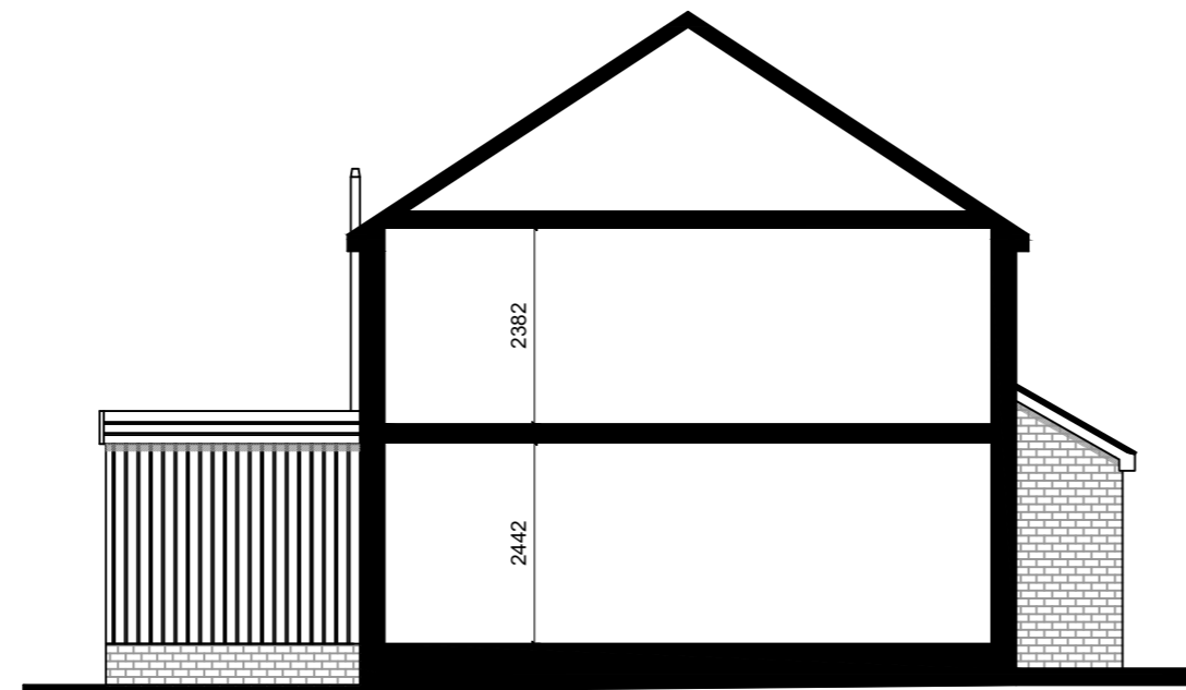
South Elevation / Section @ 1:100 scale
