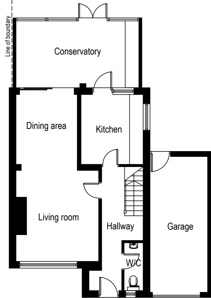
Ground floor plan @ 1:100 scale
