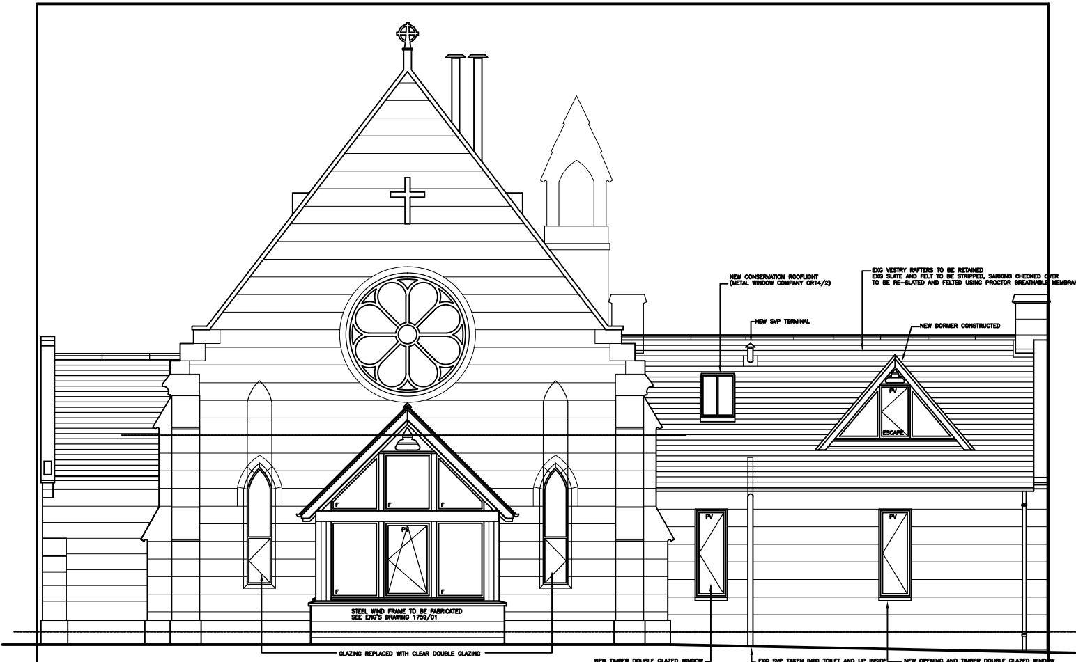
WEST ELEVATION SCALE 1 : 50
