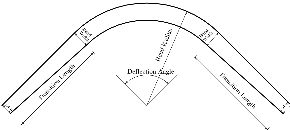
Bend Widening
