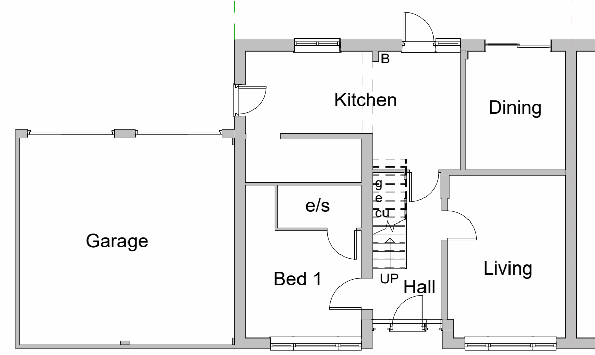
① Existing Ground Floor 1:100
