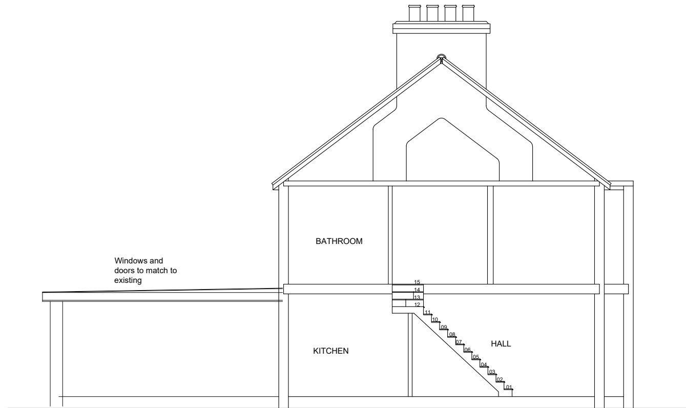
PROPOSED SECTION
