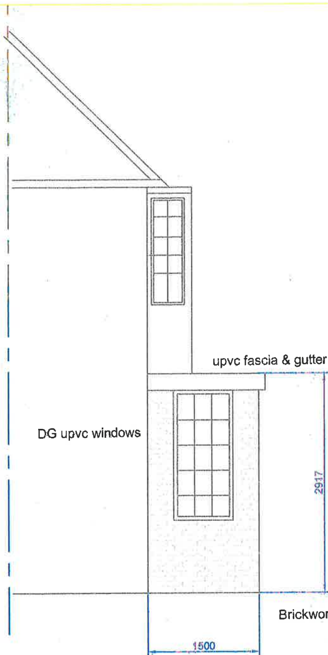
PROPOSED PART SIDE ELEVATION
