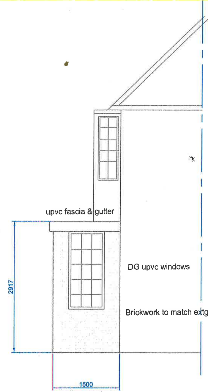
PROPOSED PART SIDE ELEVATION
