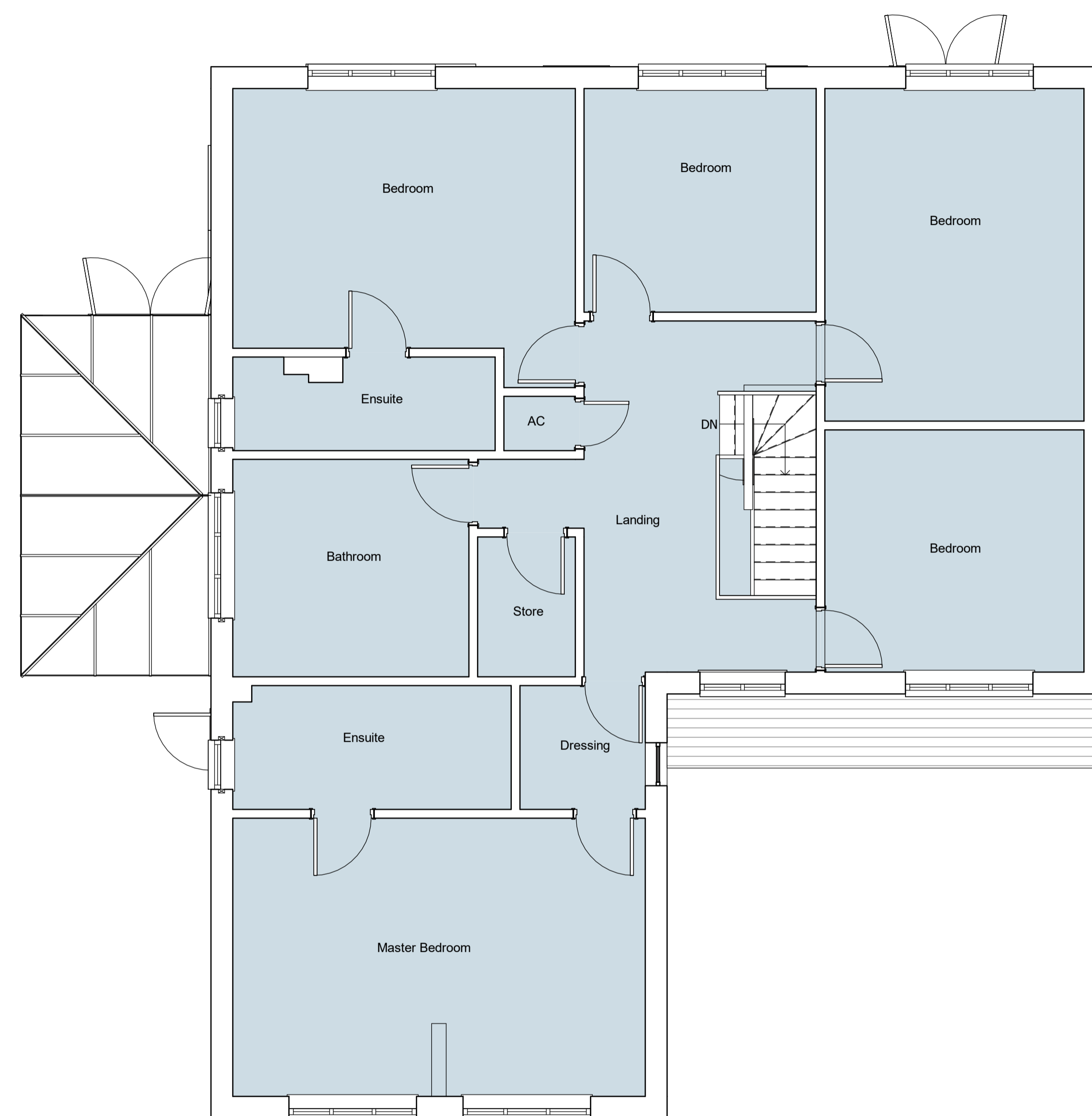
01 First Floor 1 : 50
