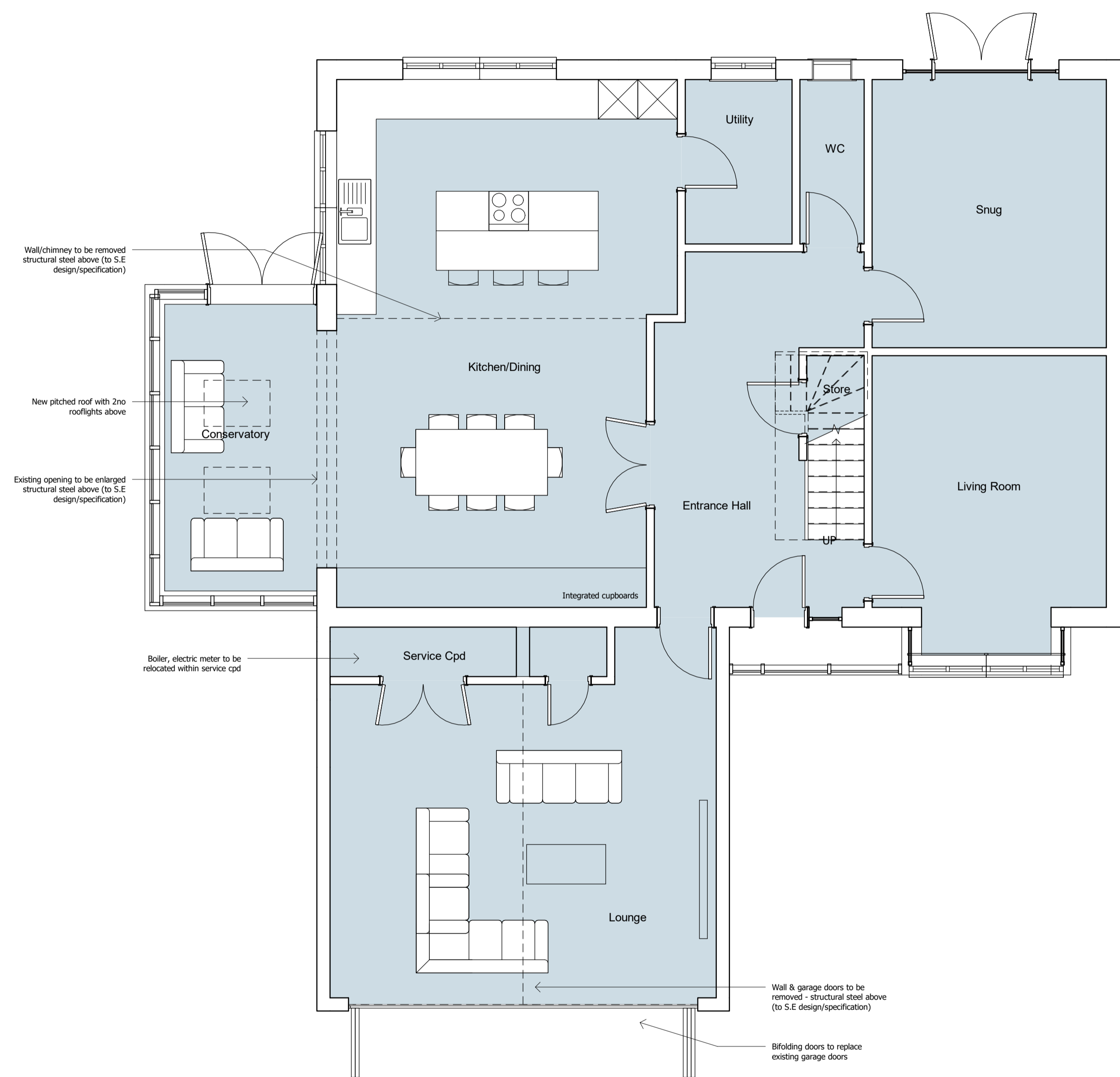
00 Ground Floor 1 : 50
