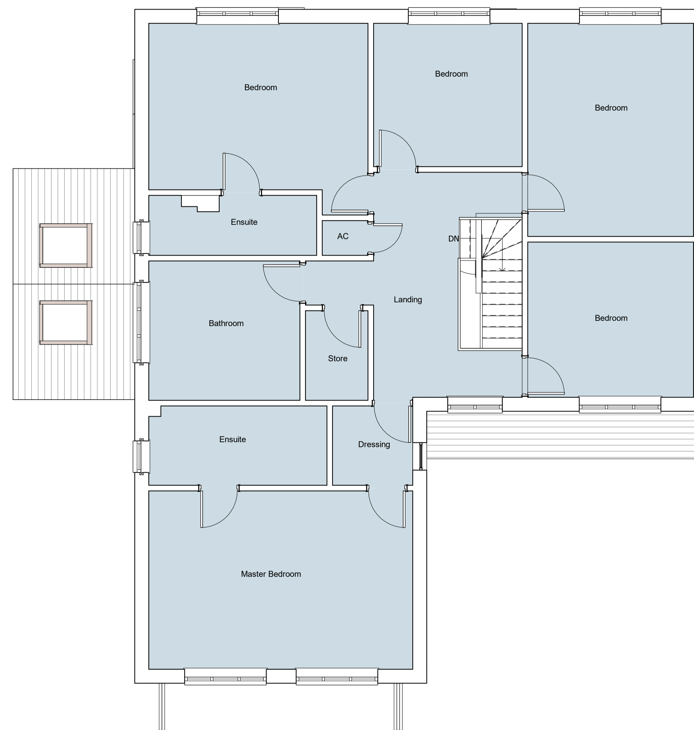
01 First Floor. 1 : 50
