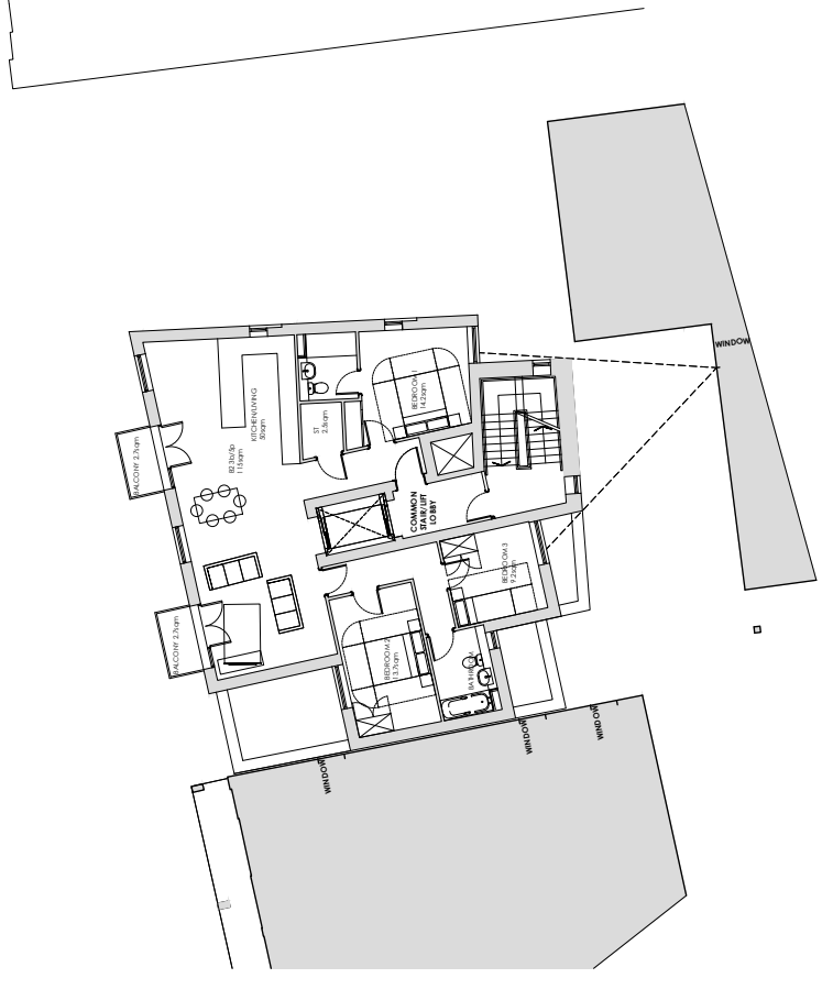
FIFTH FLOOR
