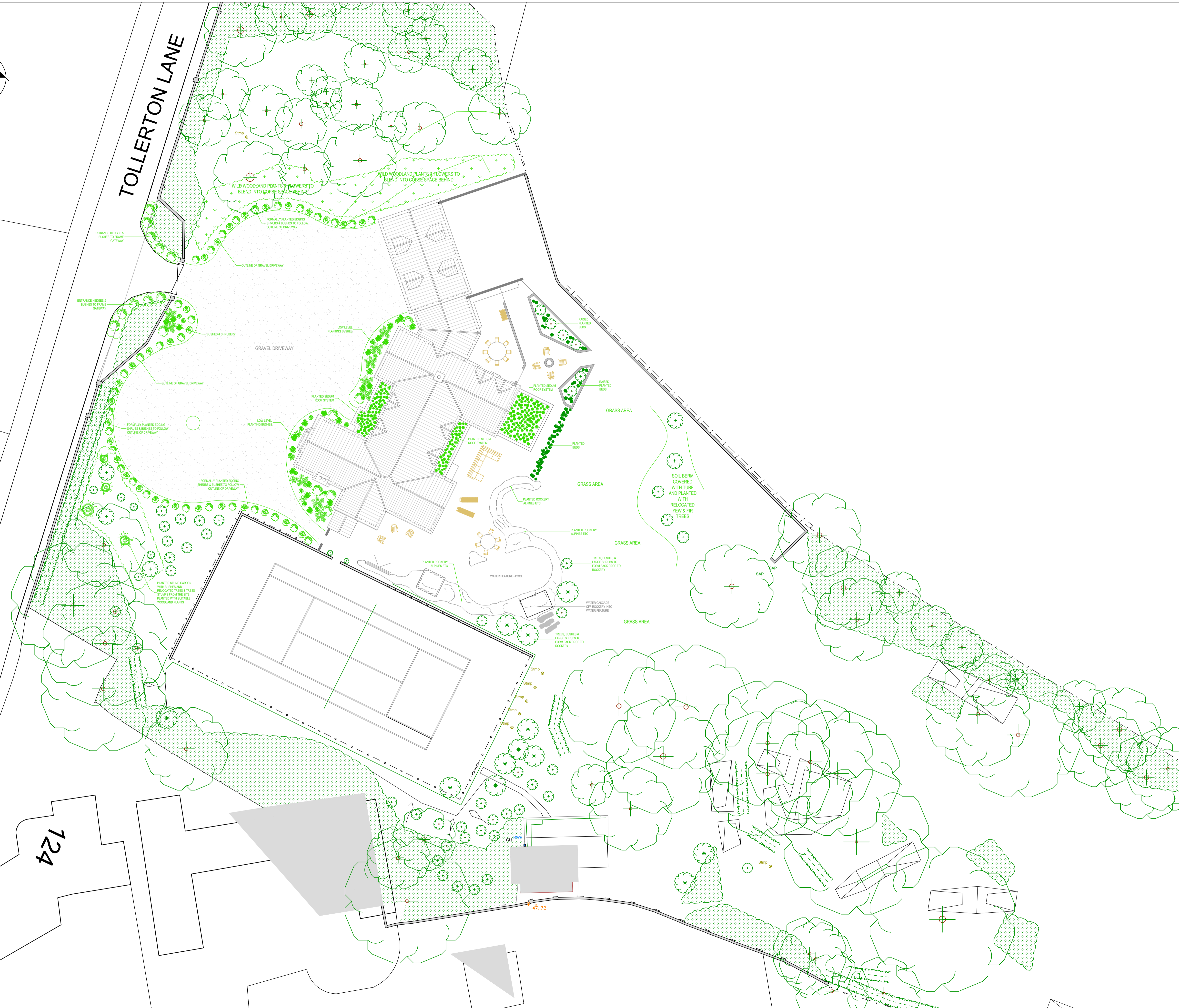
Proposed Site Layout Plan (1:200)
