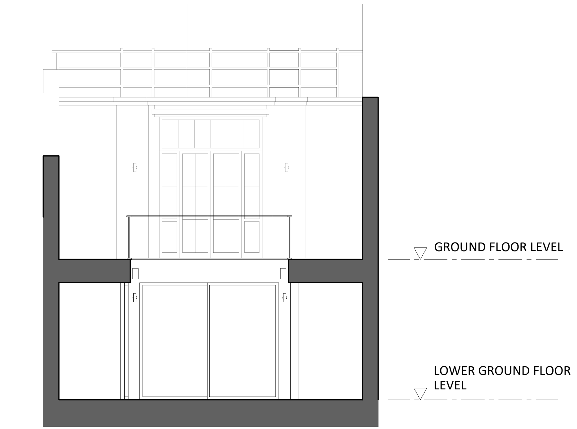
ELEVATION 'A'
