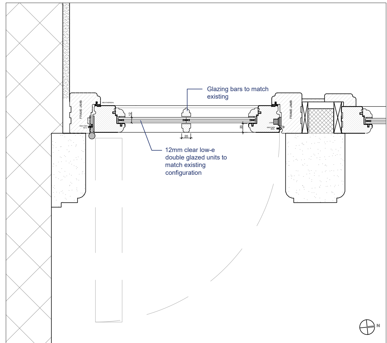
PROPOSED DETAIL FOR NEW BALCONY DOOR
