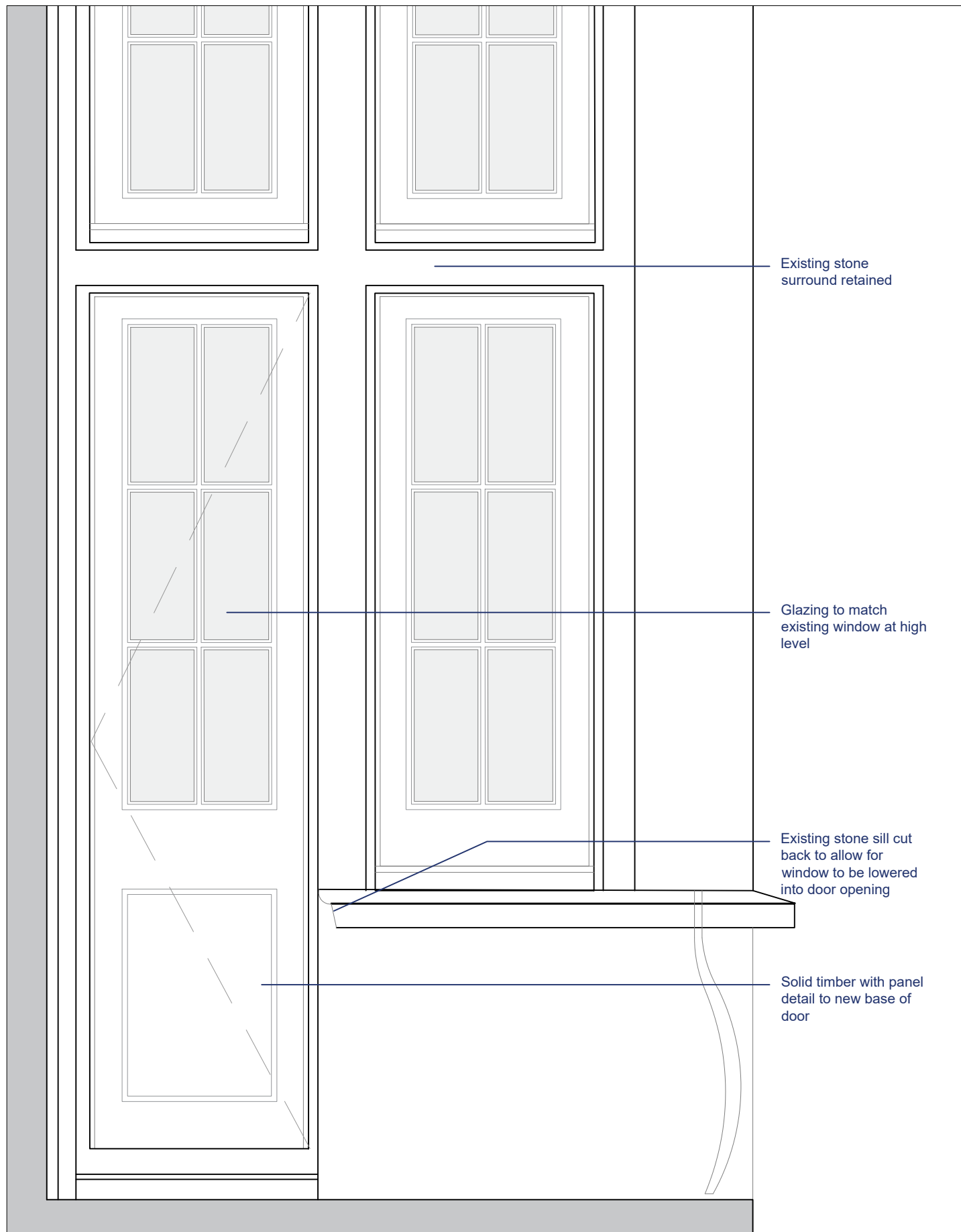
PROPOSED DETAIL ELEVATION OF NEW BALCONY DOOR
