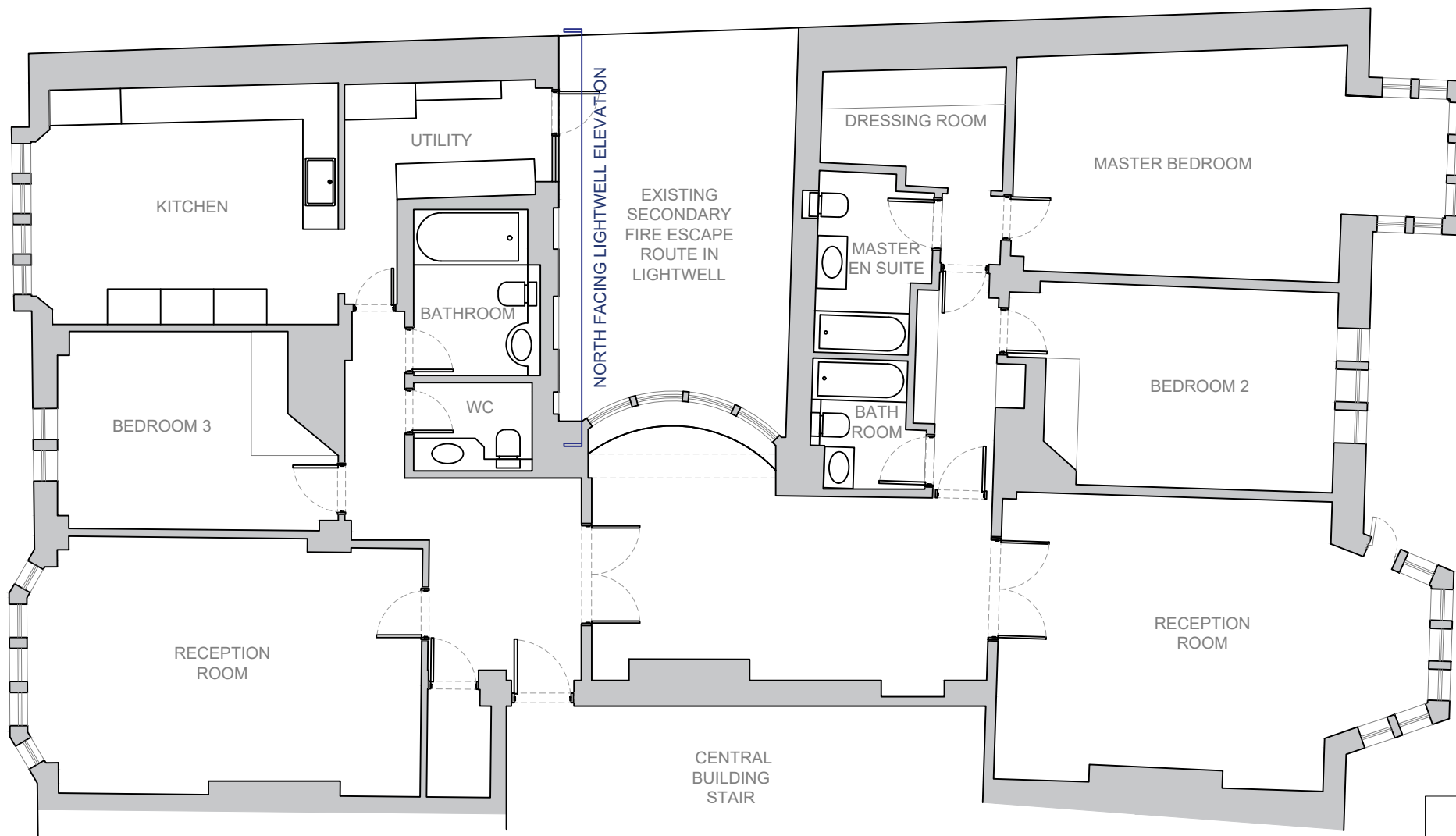
EXISTING PLAN 1/100
