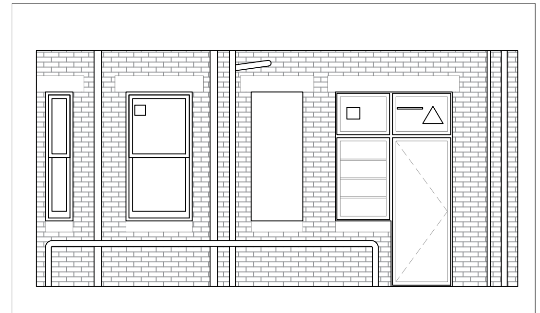
EXISTING NORTH FACING LIGHTWELL ELEVATION 1/50
